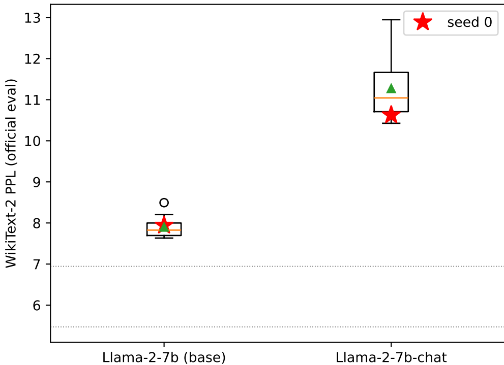
Random-Hadamard W4A4KV16 RTN: 10-seed distribution
