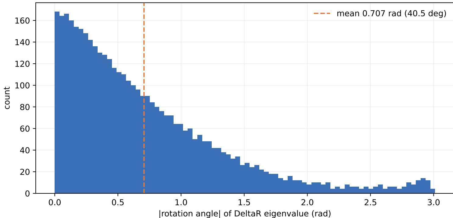
C8 DeltaR eigen-angle distribution — NOT a small correction
