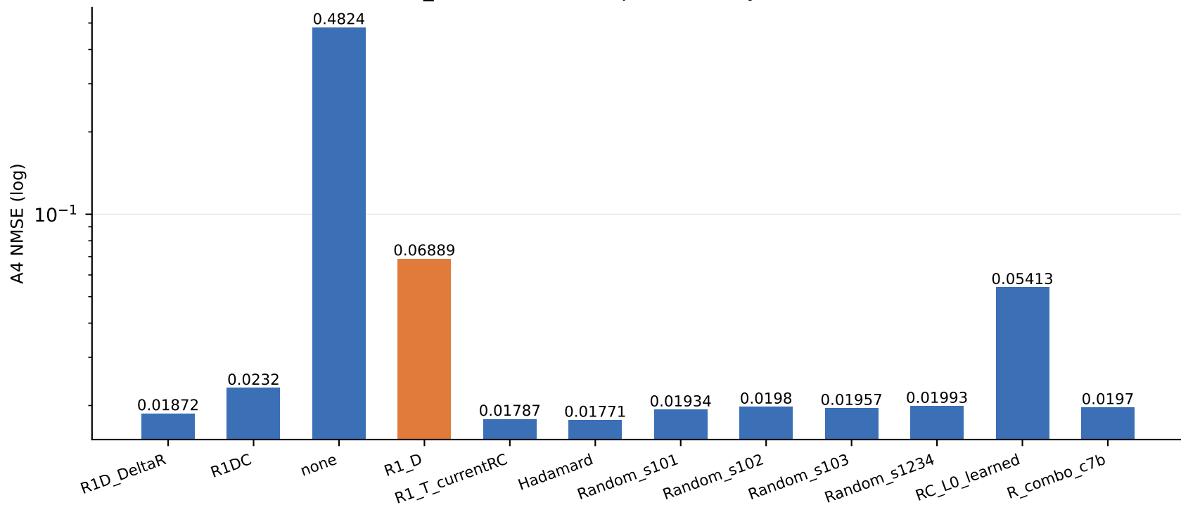
H_t A4 NMSE (mean per-token) by candidate
