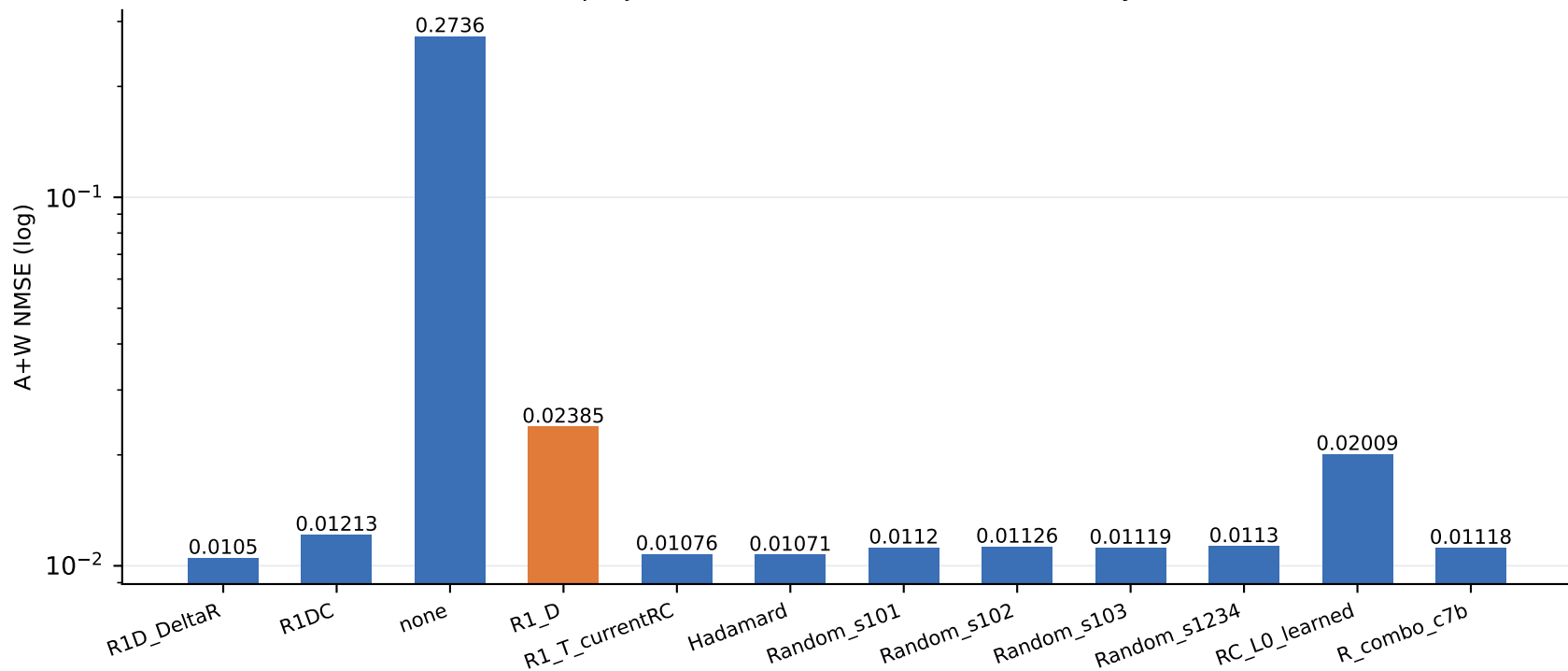
ctx K projection W4A4 NMSE (mean over 5 layers)
