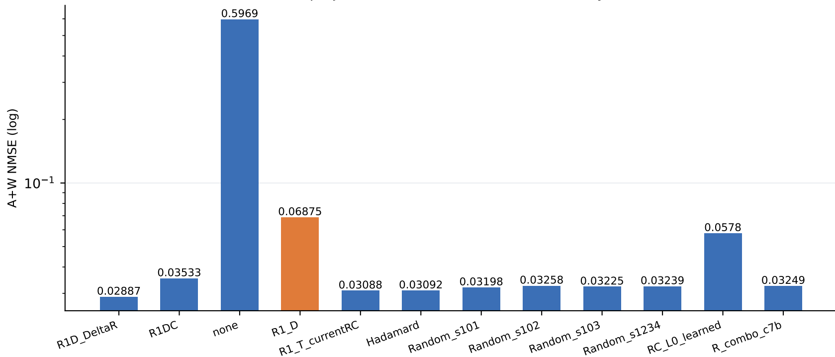
ctx V projection W4A4 NMSE (mean over 5 layers)
