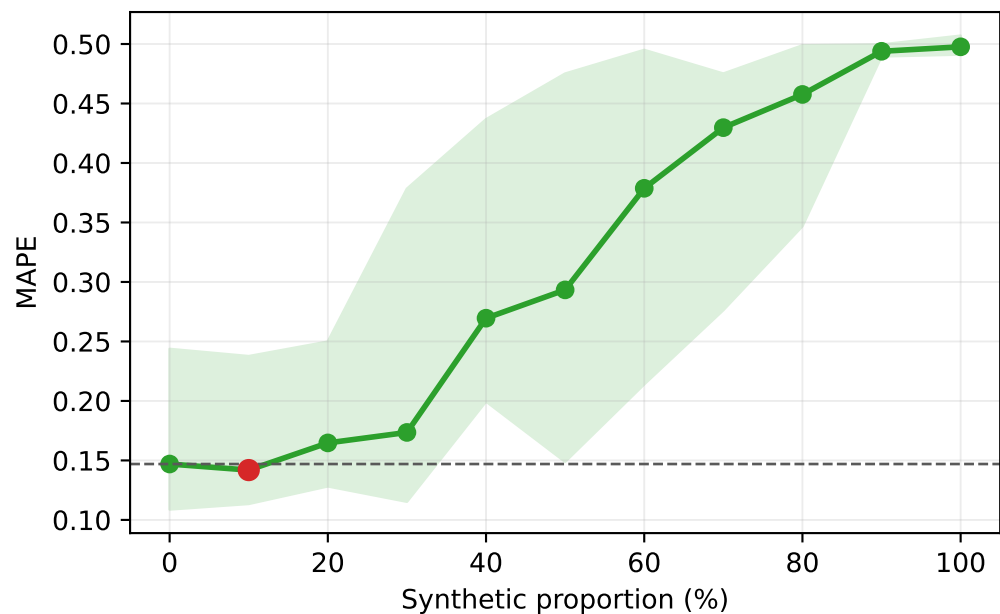
TMTR Prices
