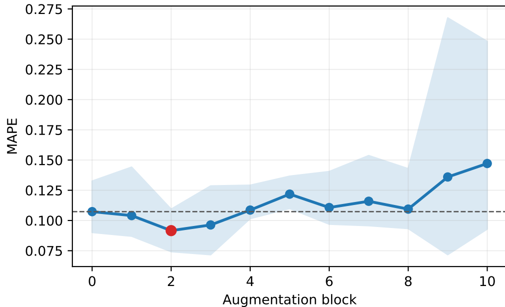
TATR Prices
