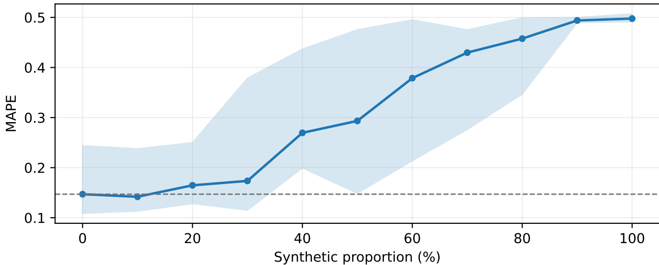
SP500 TMTR on Prices (reduced author-style run)
