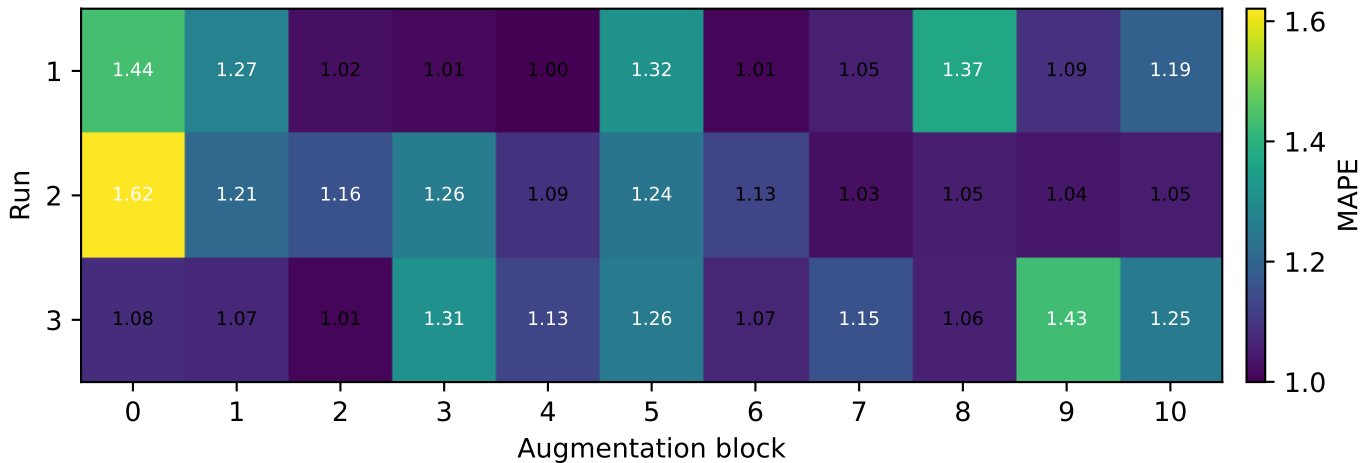
TATR Returns MAPE by Run
