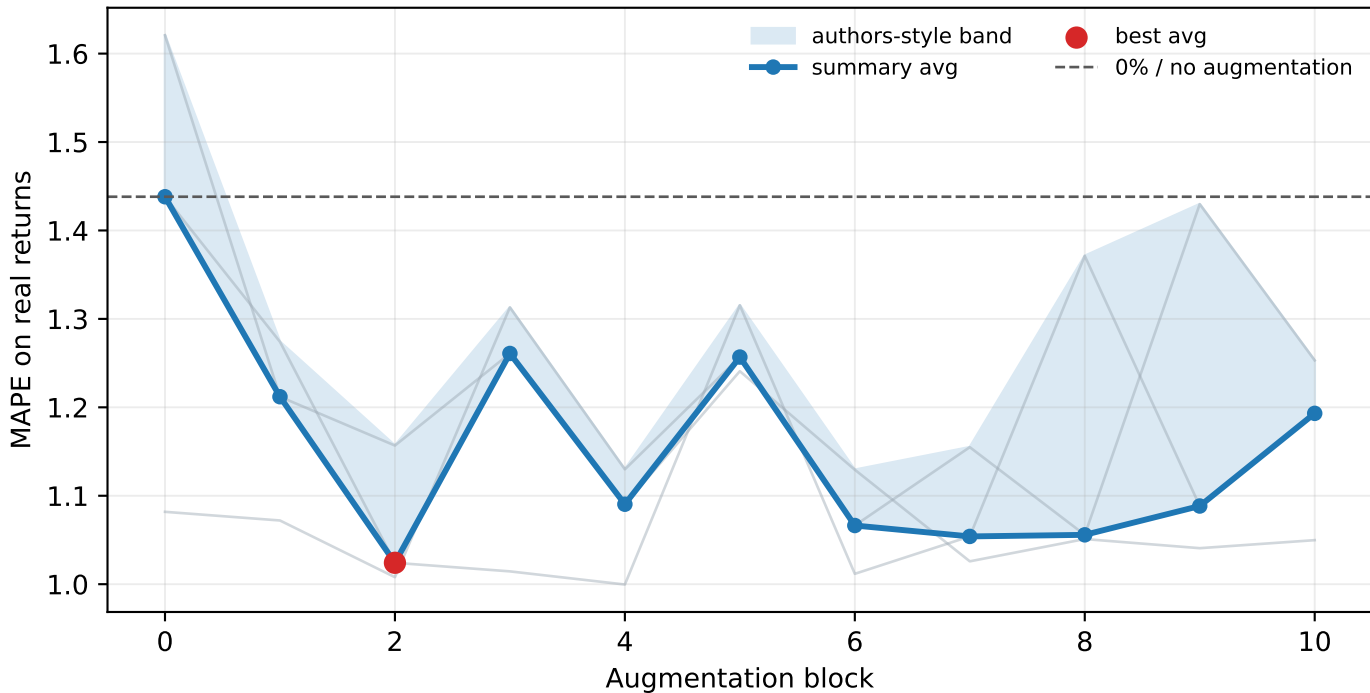
SP500 TATR on Returns
