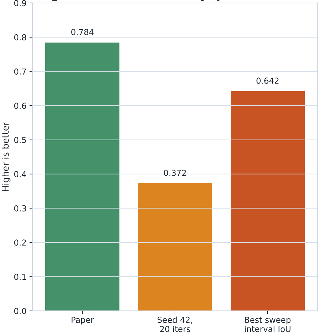
Segmentation Recovery: Jaccard / IoU
