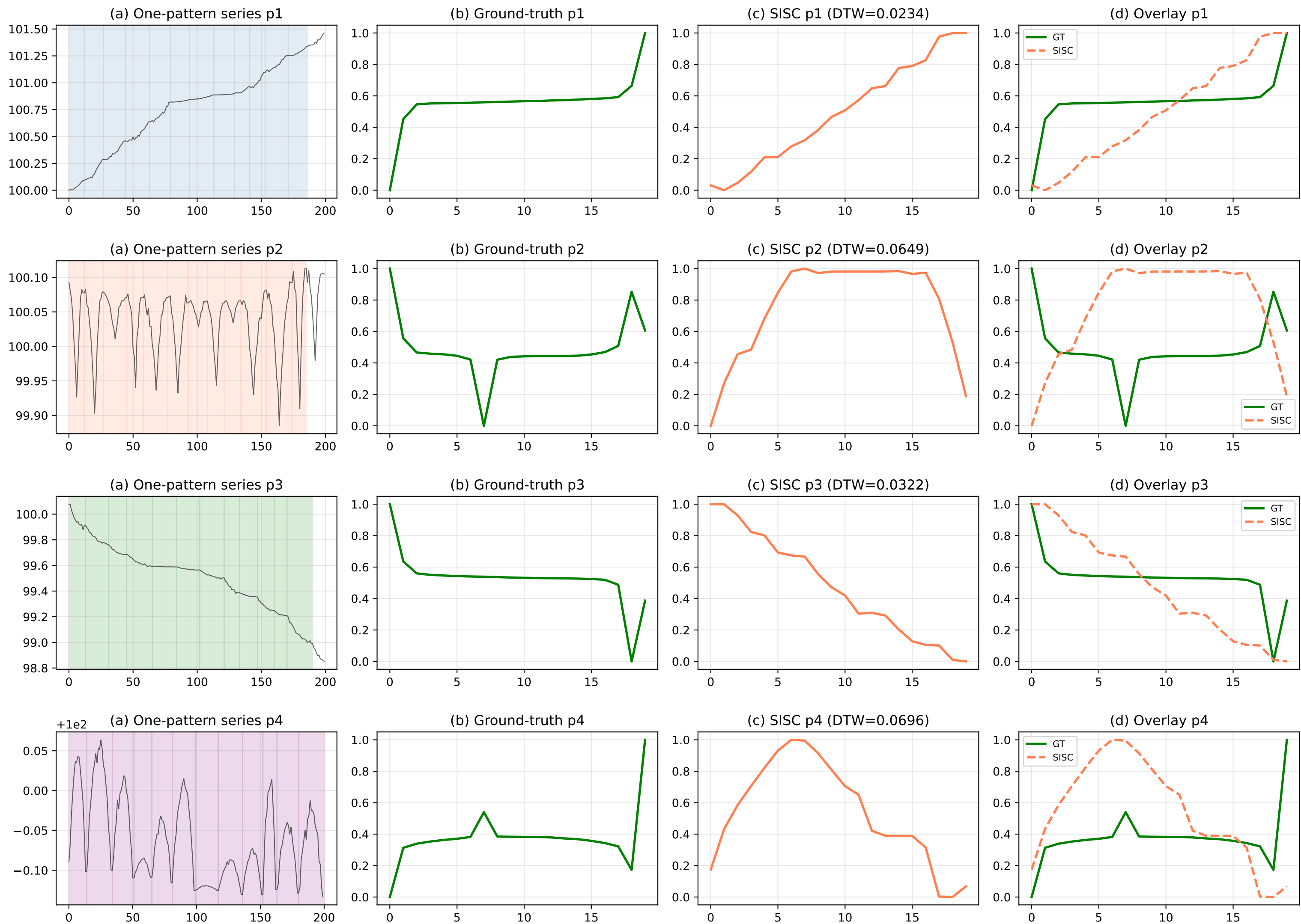
B.3 Fig. 8 replication — One-pattern (per pattern, derived from toy data) Avg per-unit DTW = 0.0475 (paper: 0.009) | Avg Jaccard = 0.3652 (paper: 0.938)
