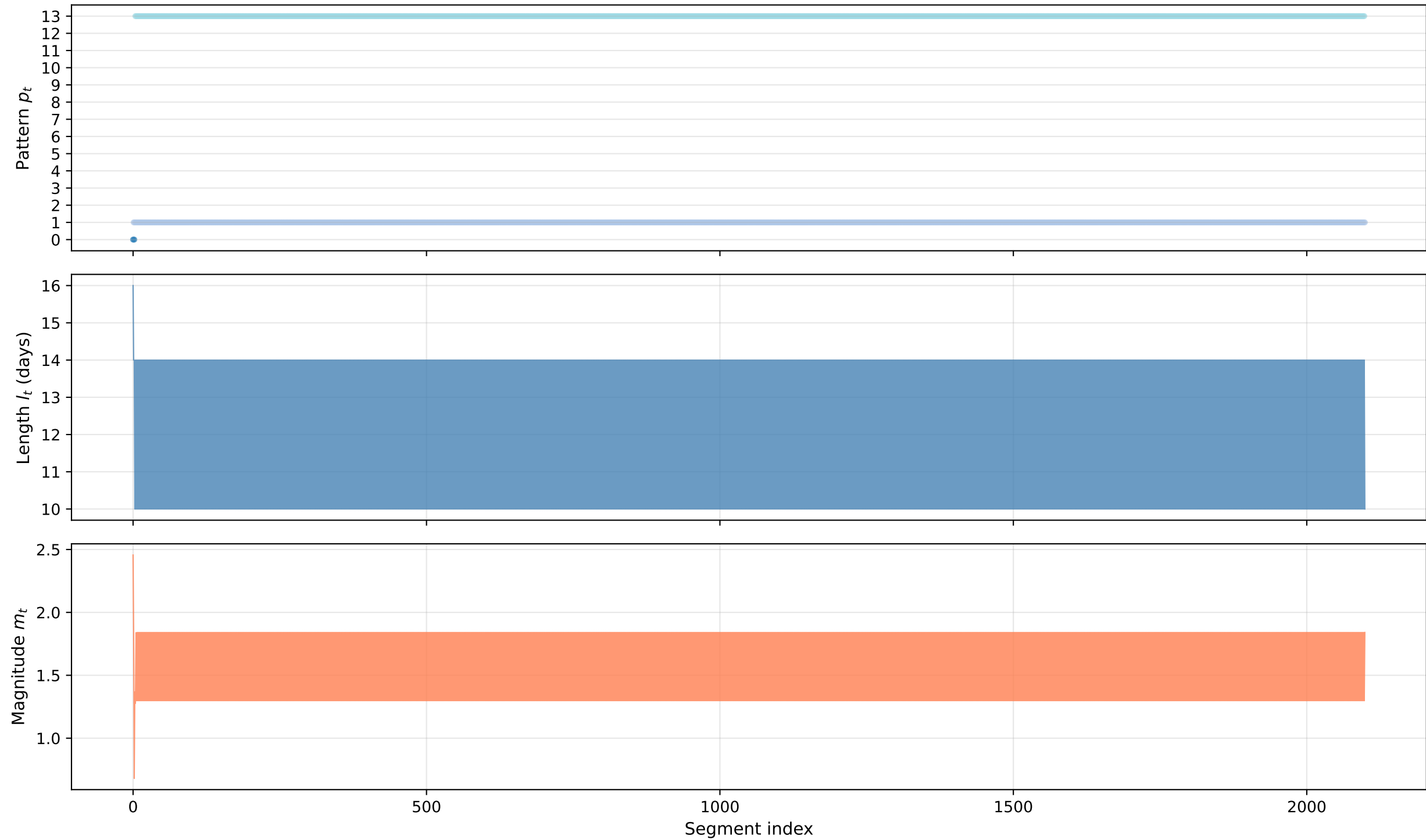
MC state evolution — GOOG K=14 'single' run 0
