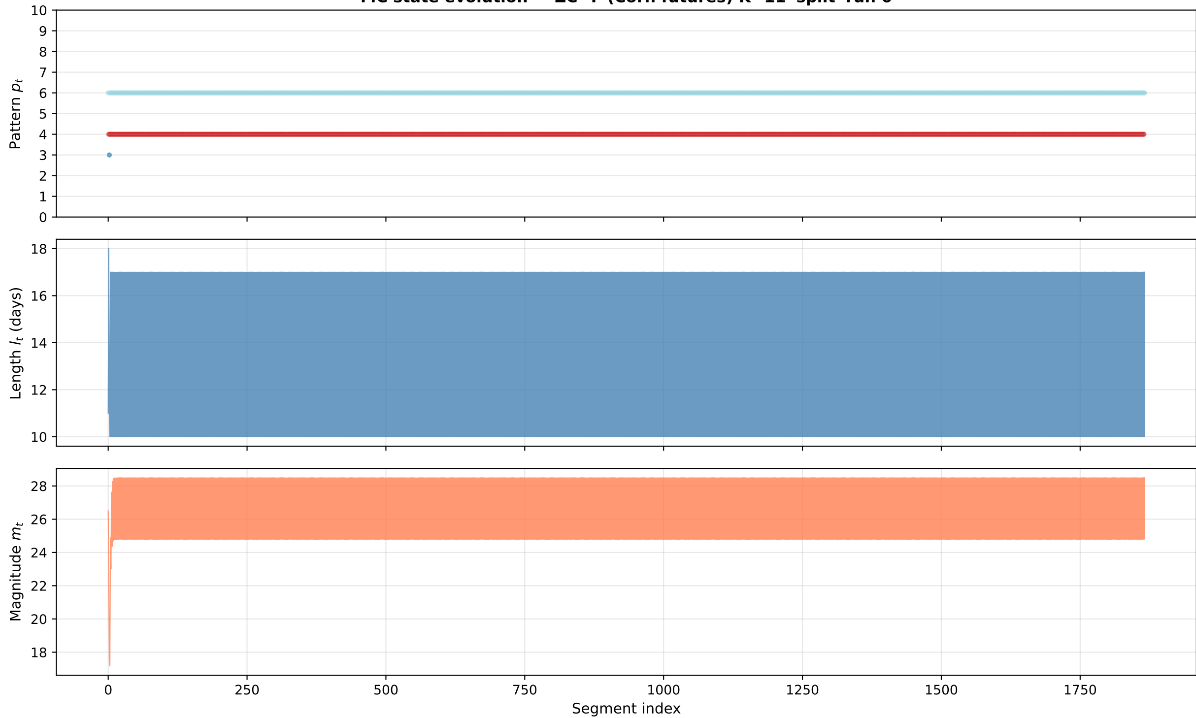
MC state evolution — ZC=F (Corn futures) K=11 'split' run 0
