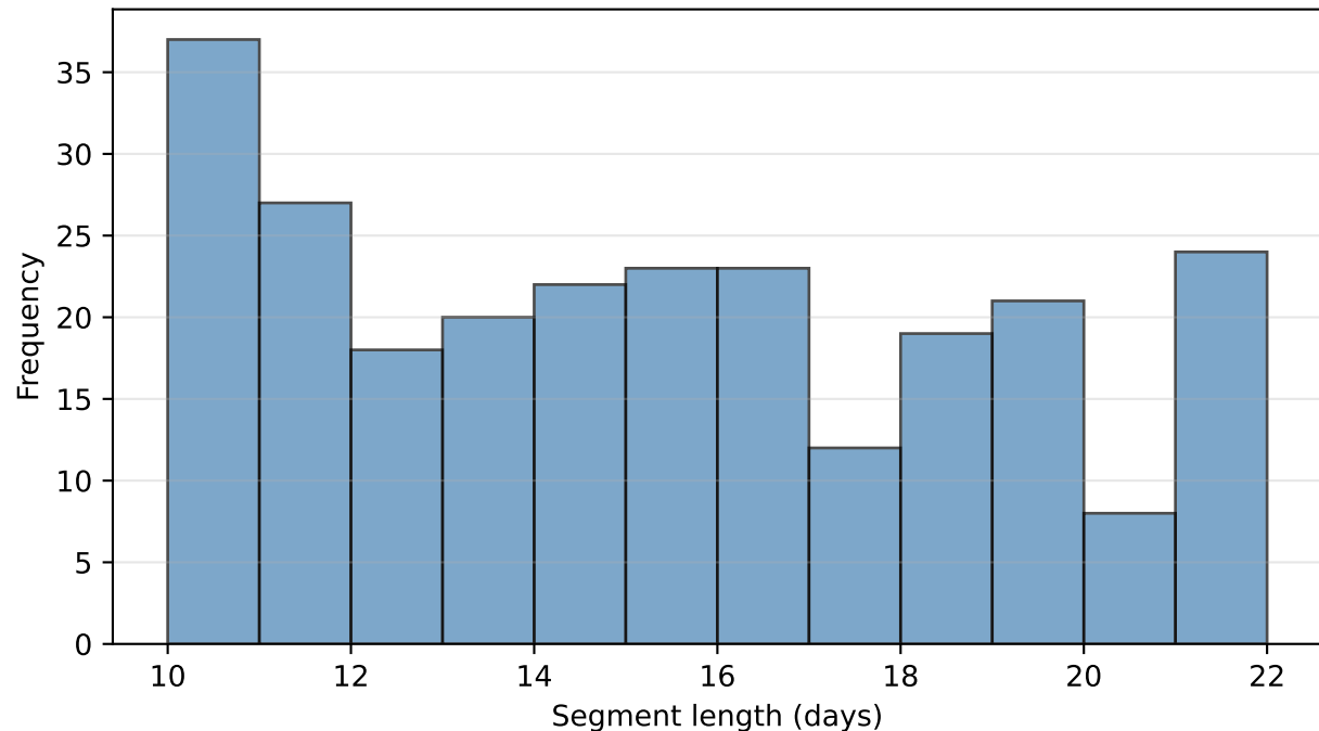
Segment length distribution (GOOG)
