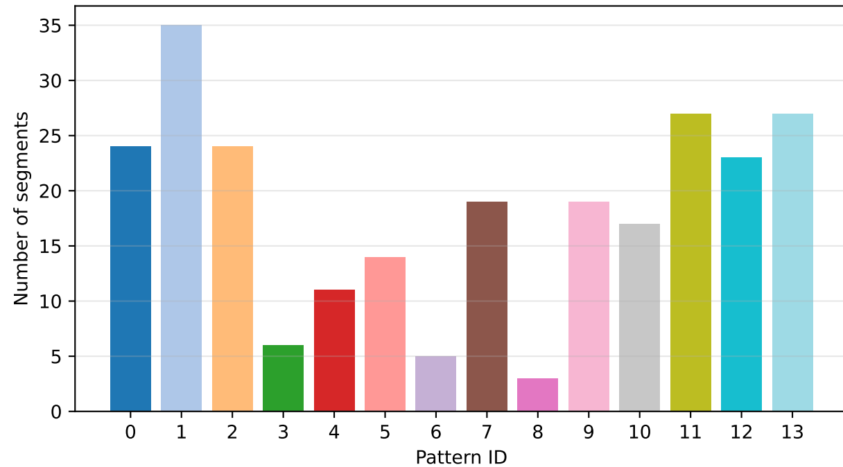
Pattern frequency (GOOG)
