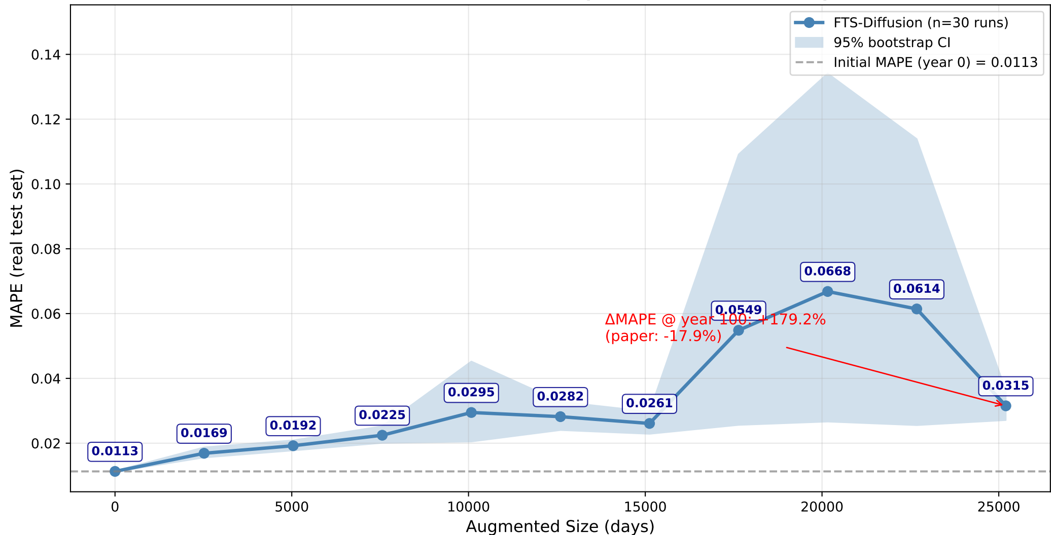
TATR — ZC=F (Corn futures) (K=11, 'split') — 30 runs × 11 eval points
