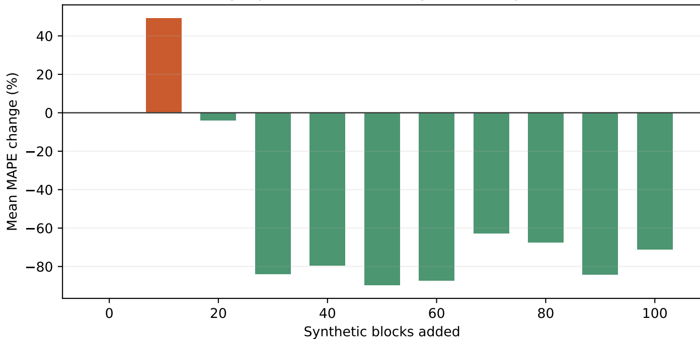
TATR single-protocol MAPE change vs no augmentation
