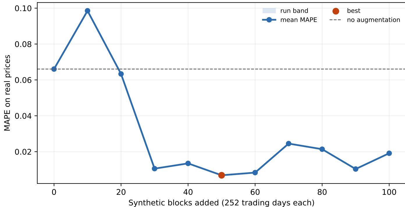
SP500 TATR on Prices, single continuous trajectory
