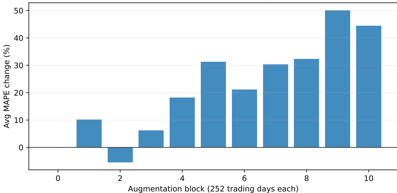
TATR price MAPE change vs no augmentation
