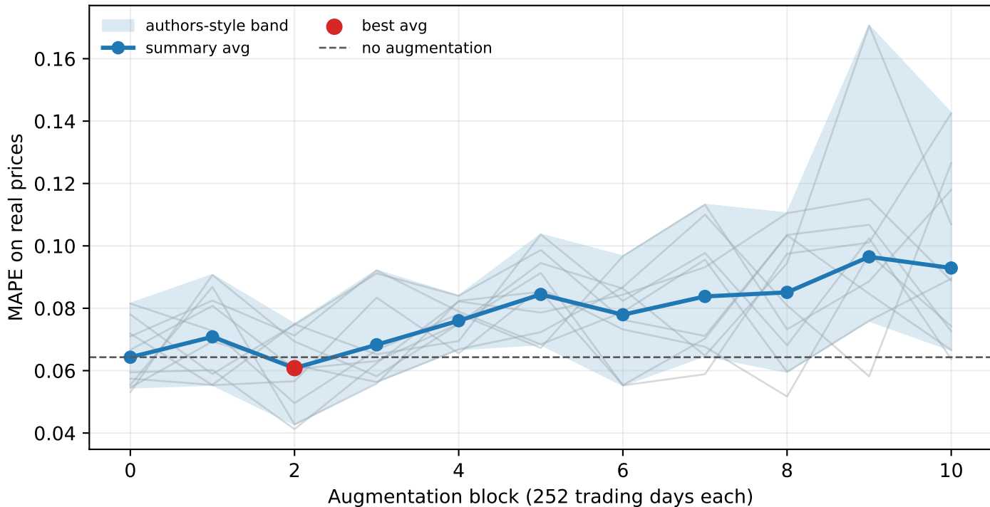
SP500 TATR on Prices, author-style reduced run
