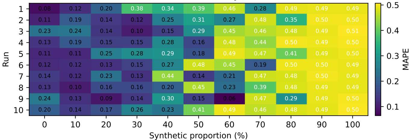
TMTR Prices MAPE by Run
