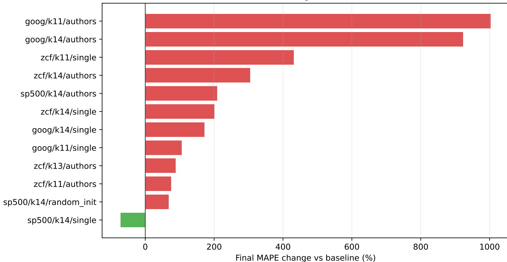
TATR Final-Point Change Across Stored Runs
