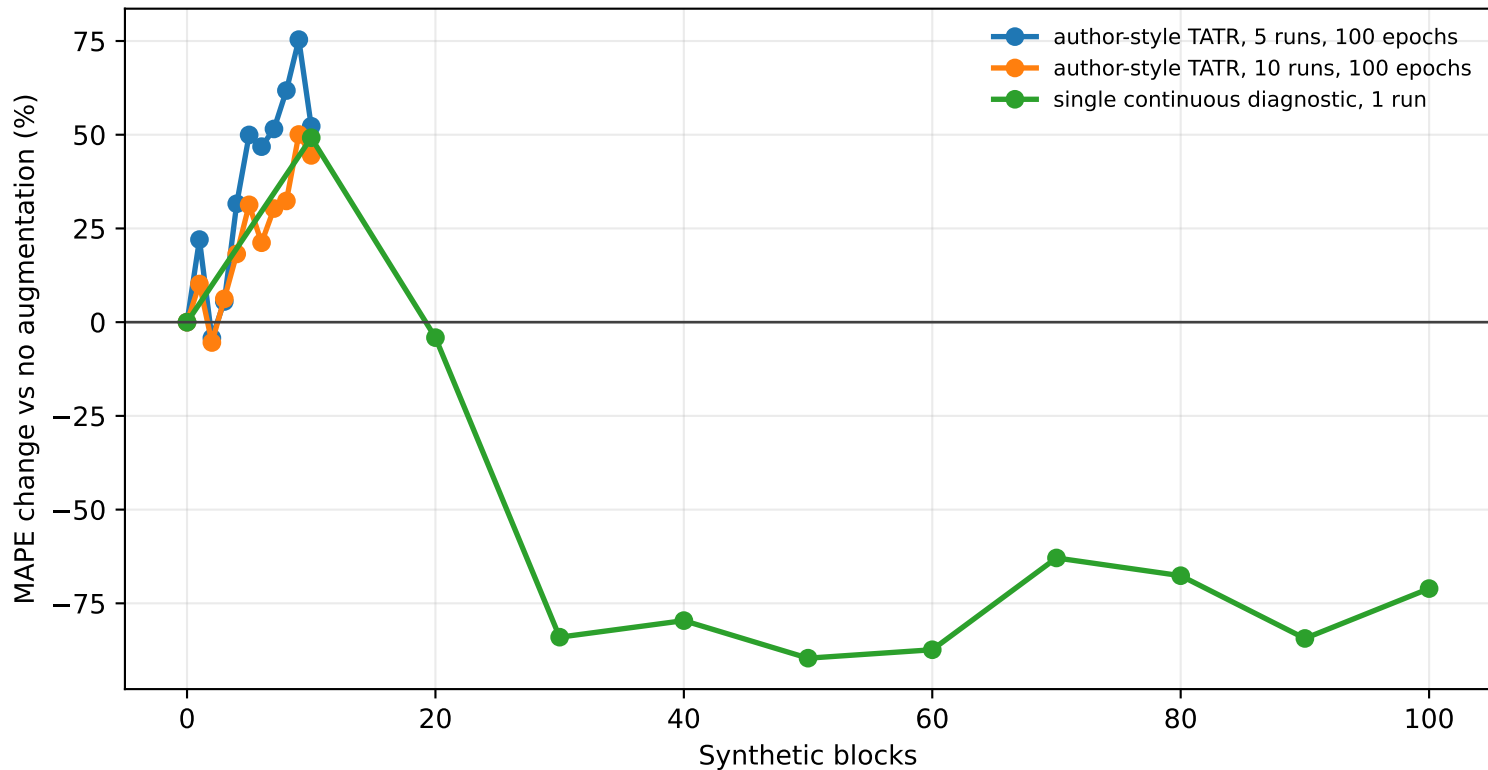
SP500 TATR: author-style curves vs single diagnostic
