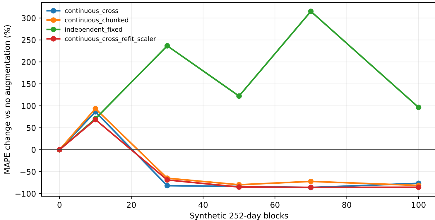
SP500 TATR protocol search
