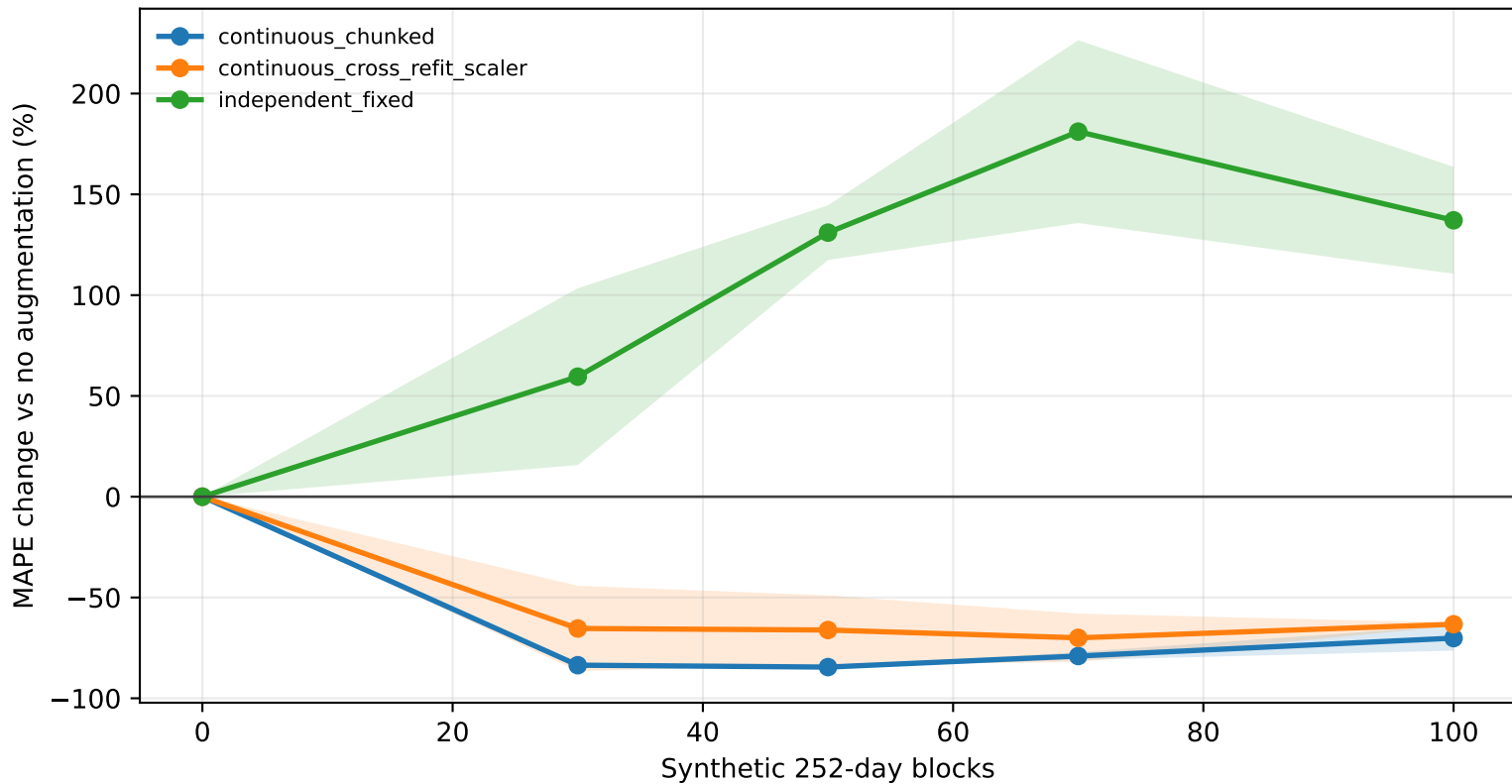
SP500 TATR multi-seed protocol robustness
