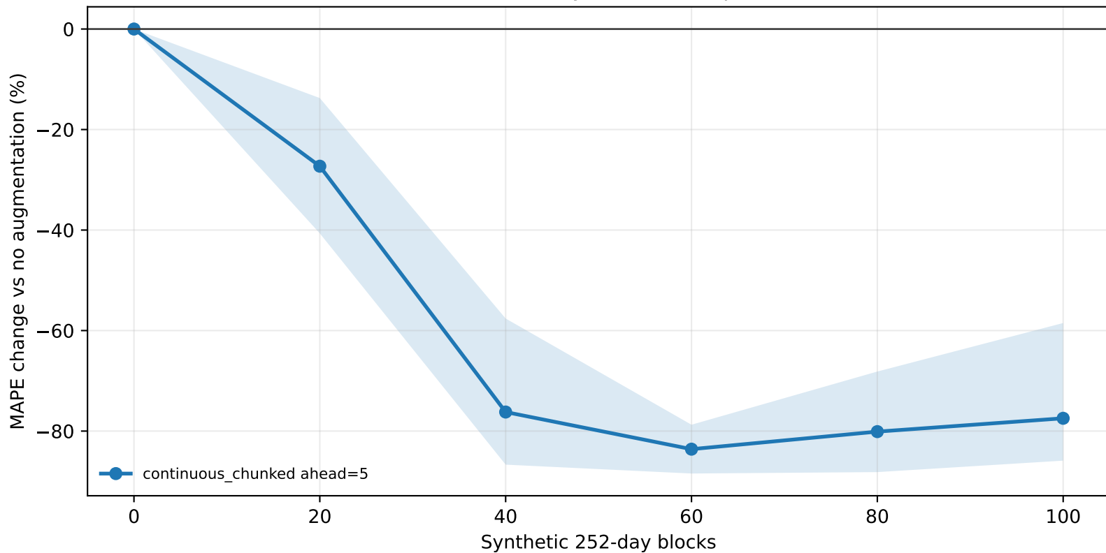
SP500 TATR 5-day continuous protocol
