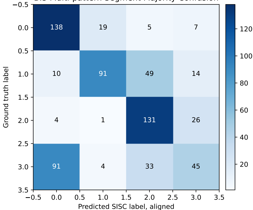
B.3 Multi-pattern Segment Majority Confusion
