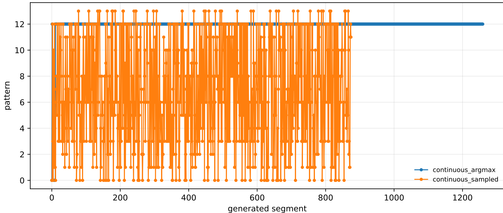
Continuous pattern paths: argmax collapse vs sampled PEM
