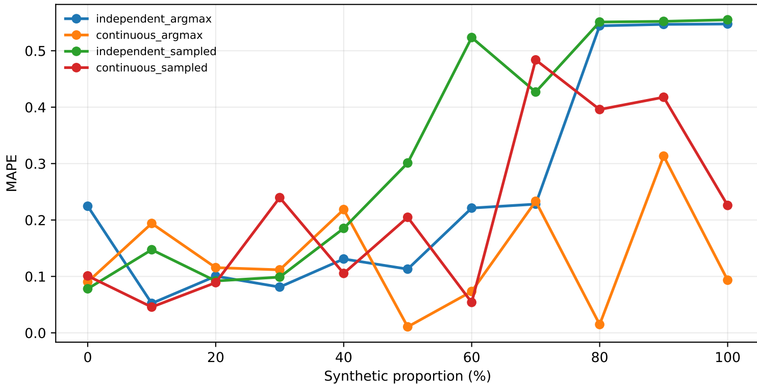
S&P 500 TMTR smoke: argmax vs sampled PEM (100 epochs)
