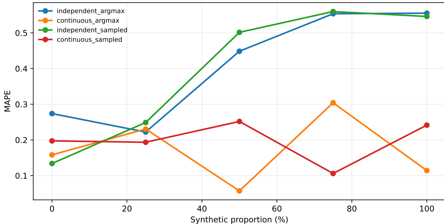
S&P 500 TMTR smoke: argmax vs sampled PEM (30 epochs)
