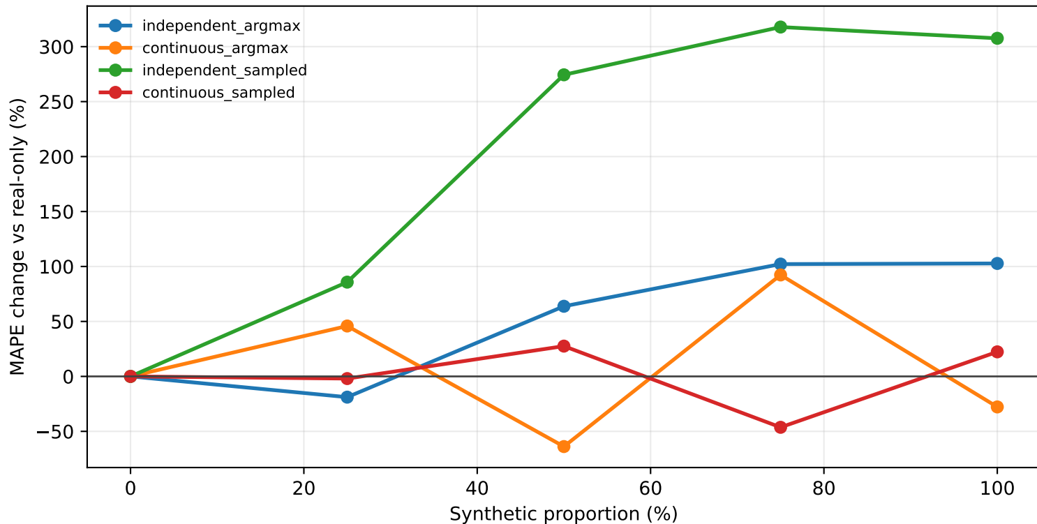
S&P 500 TMTR smoke change vs real-only (30 epochs)
