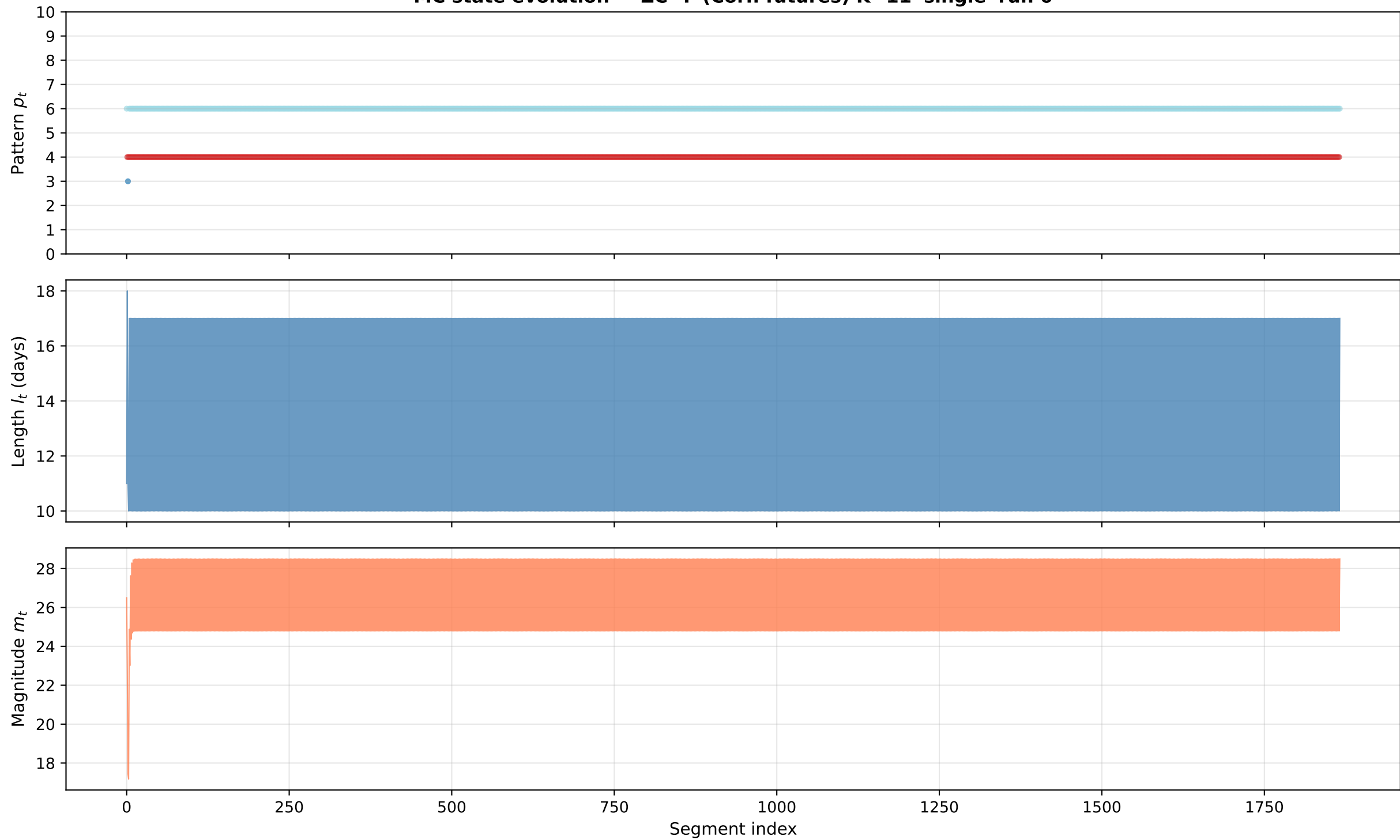
MC state evolution — ZC=F (Corn futures) K=11 'single' run 0
