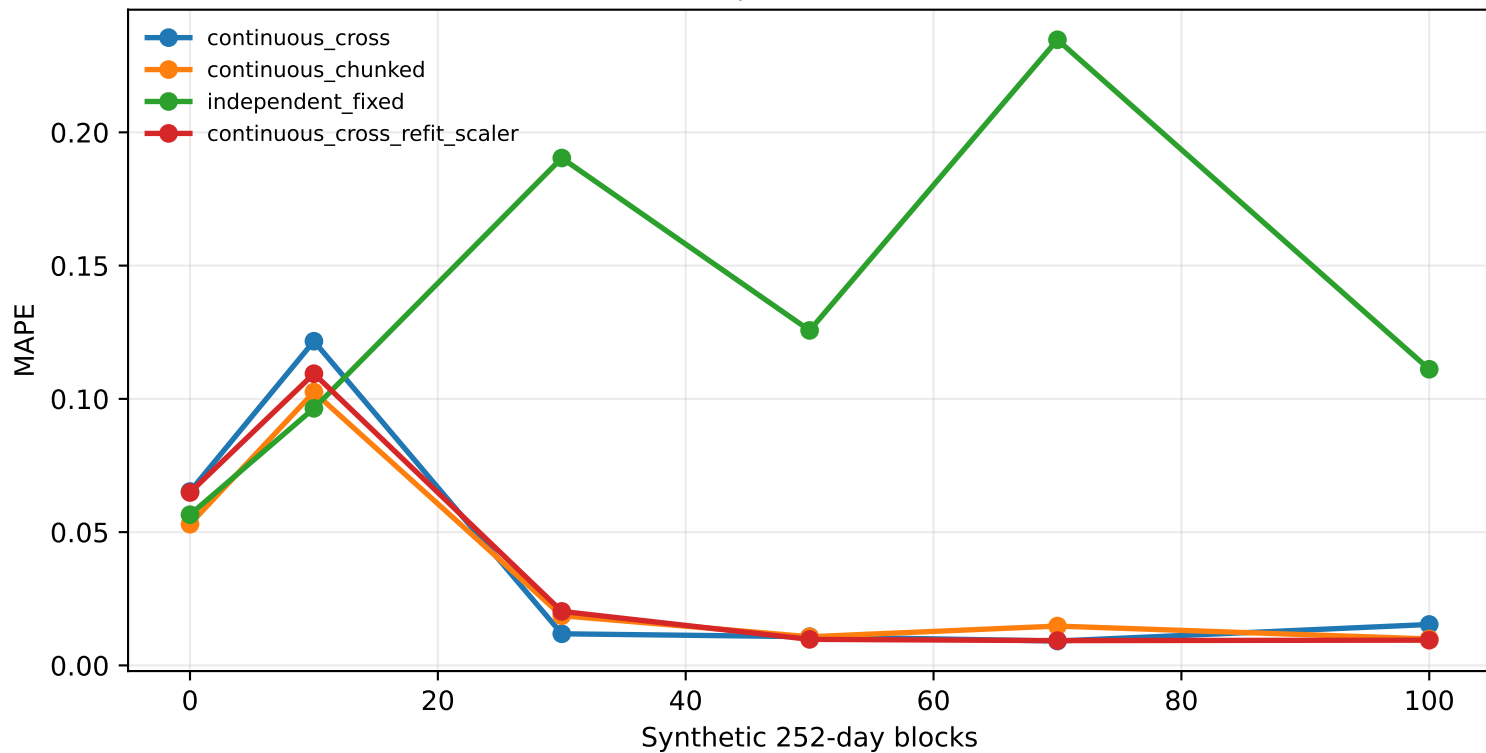
SP500 TATR protocol search MAPE
