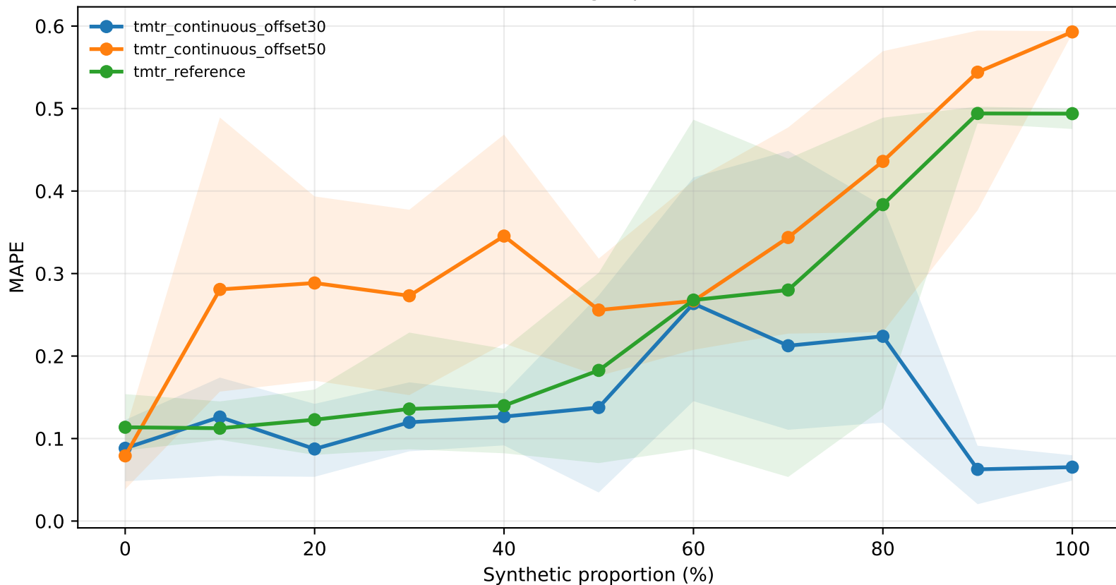
SP500 TMTR: long replication batch
