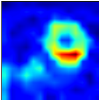
Grad-CAM
