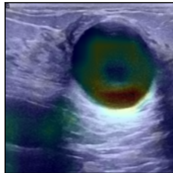
Overlay
