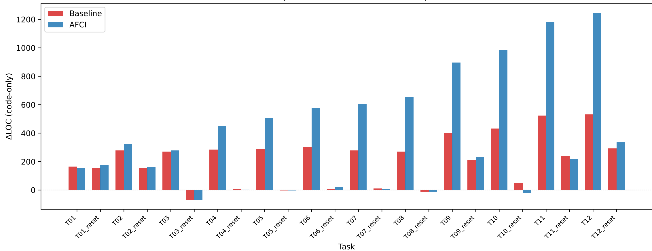
Code-Only Drift: Baseline vs AFCI (v1, Opus 7)
