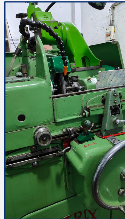
Universal Thread Grinding Machine (Make: Matrix, Model: 16 U)
