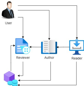
Fig. 4: User Roles.
