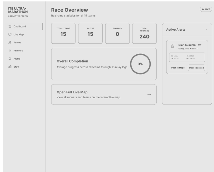
Gambar IV.26 Halaman Dashboard Panitia
