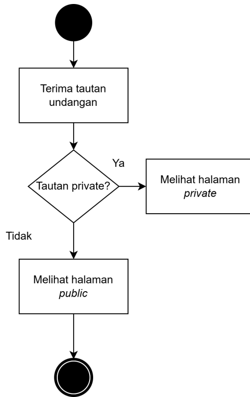
Gambar IV.17 User Flow Penonton
