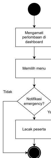
Gambar IV.16 User Flow Panitia
