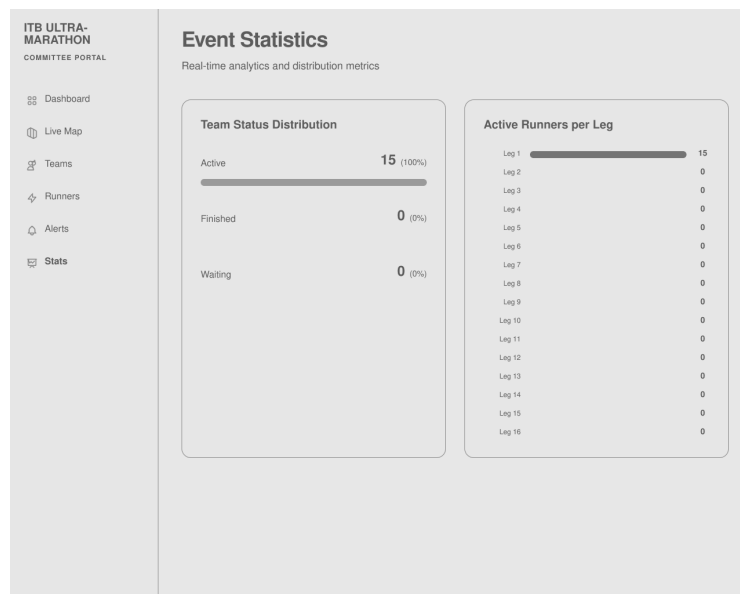
Gambar IV.30 Halaman Statistik Panitia
