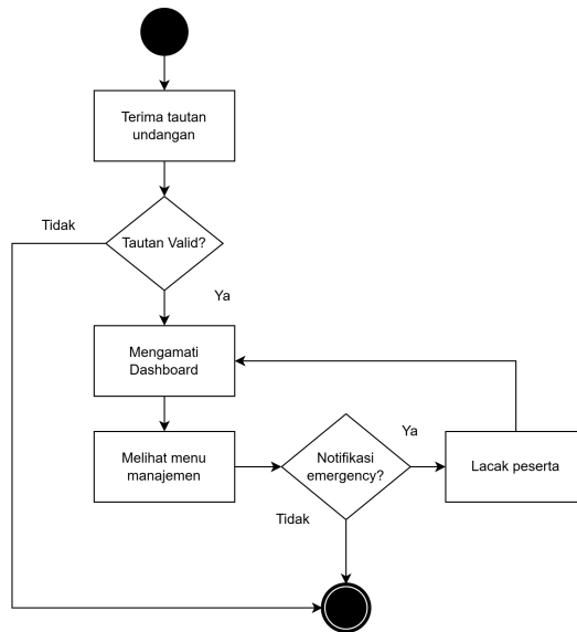
Gambar IV.15 User Flow Supporter
