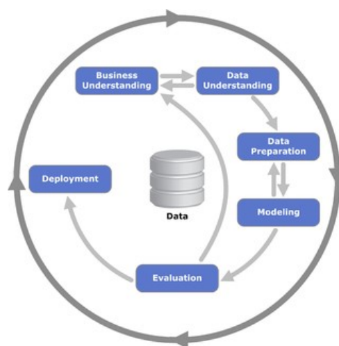
Gambar I.1 Metodologi CRISP-DM
