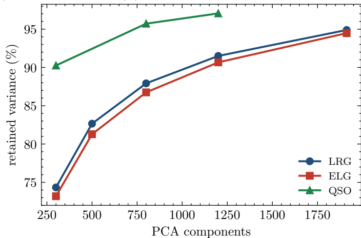
(b) variance keeps rising
