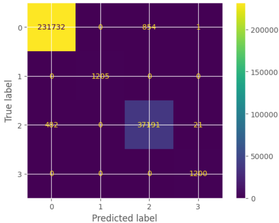
Figure 4.1: Confusion matrix for Best ANN.
