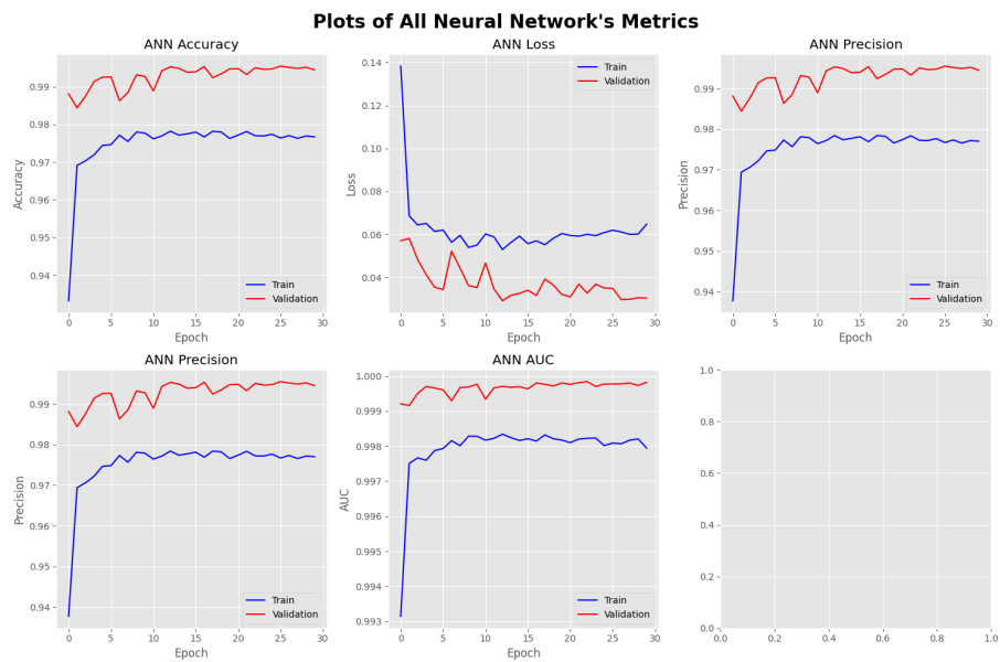
Figure 4.2: Training and validation curves for Best ANN.
