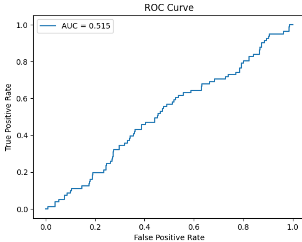
Figure 2: ROC curve for the hotspot classification model. The AUC value indicates the model barely performs better than random guessing.
