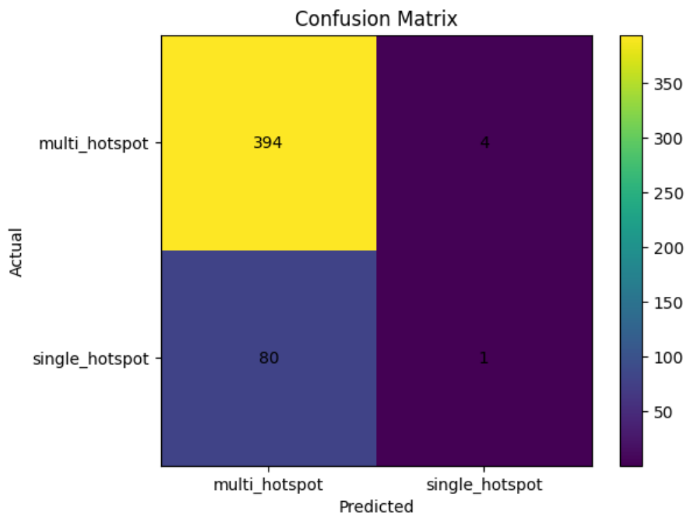
Figure 1: Confusion matrix showing the performance of the hotspot classification model. The model performs well for multiple hotspots but poorly for single hotspots
