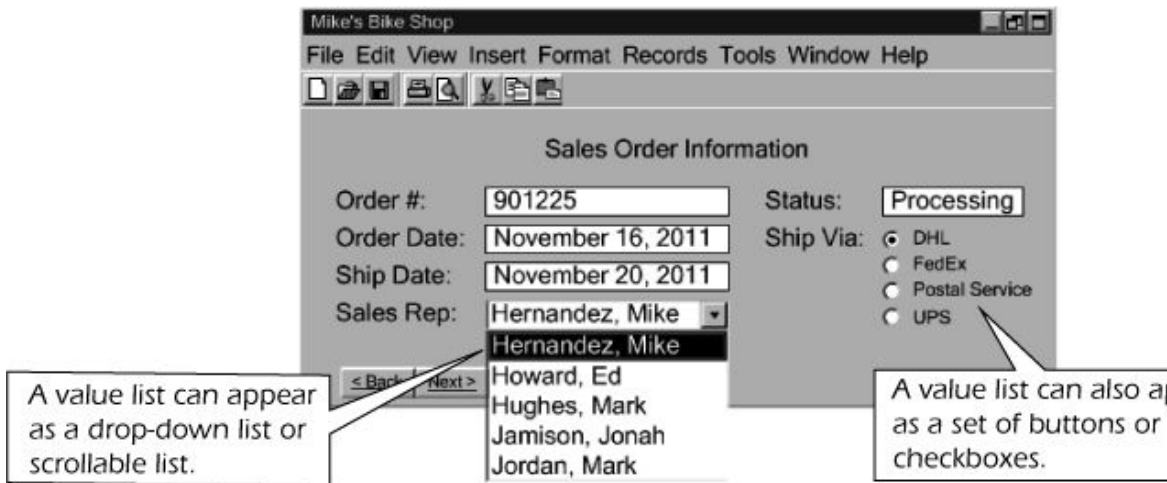
Figure 6.16. A database screen with two value lists
