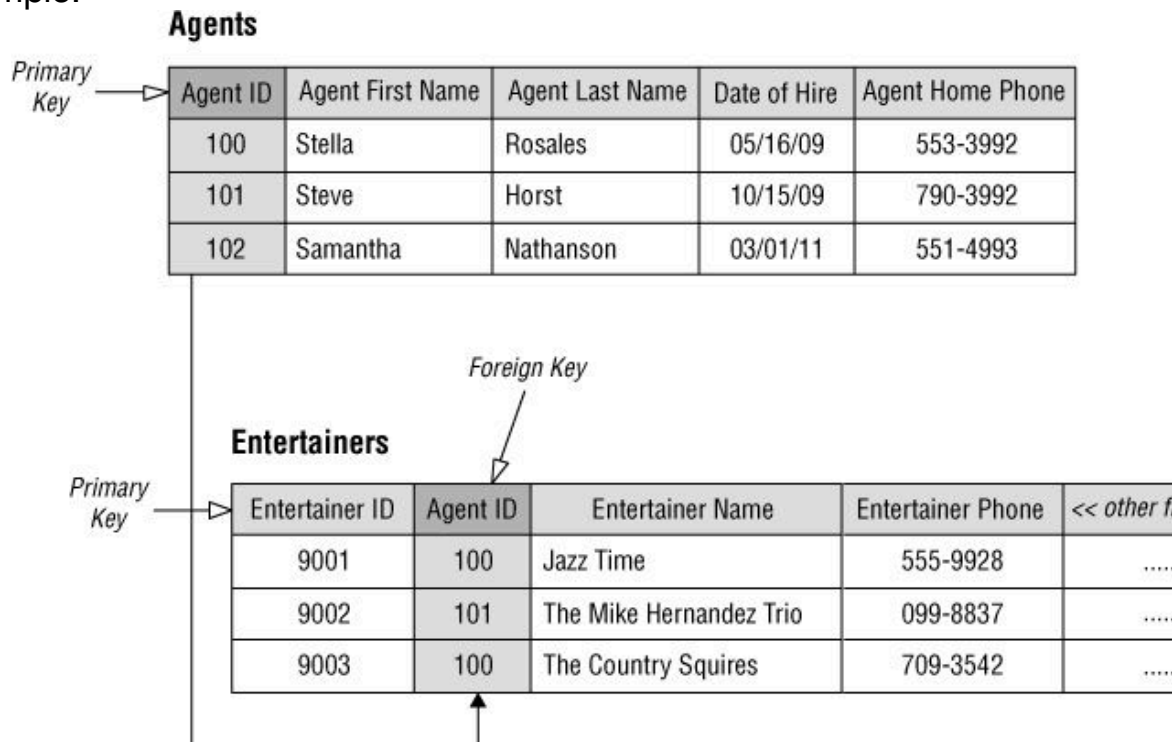
Figure 3.11. An example of primary and foreign key fields
