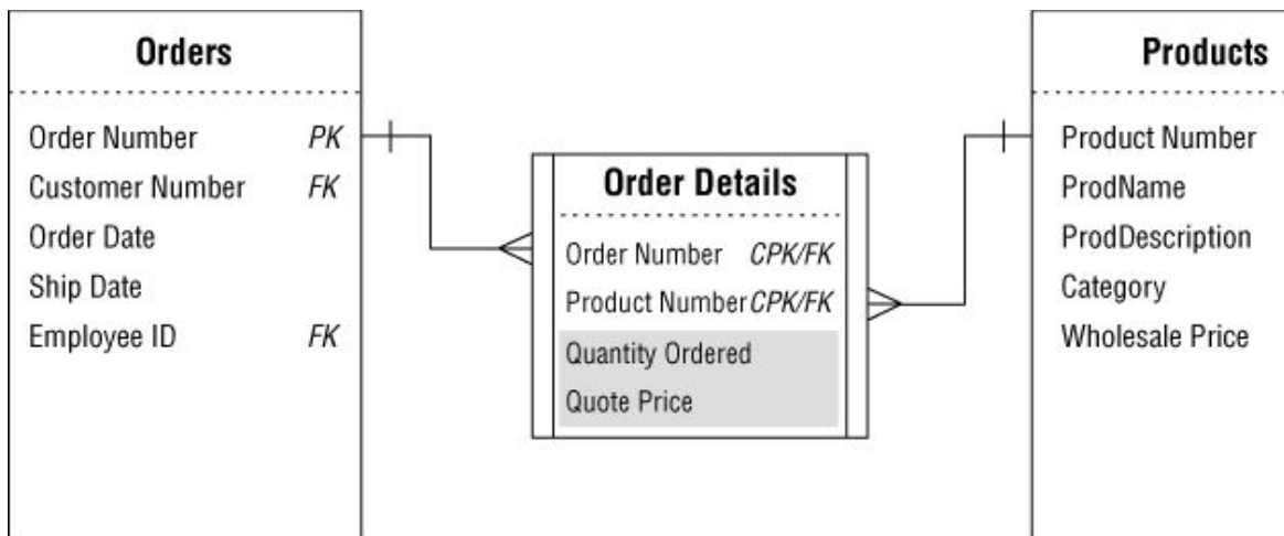
Figure 10.44. The revised ORDER DETAILS linking table
