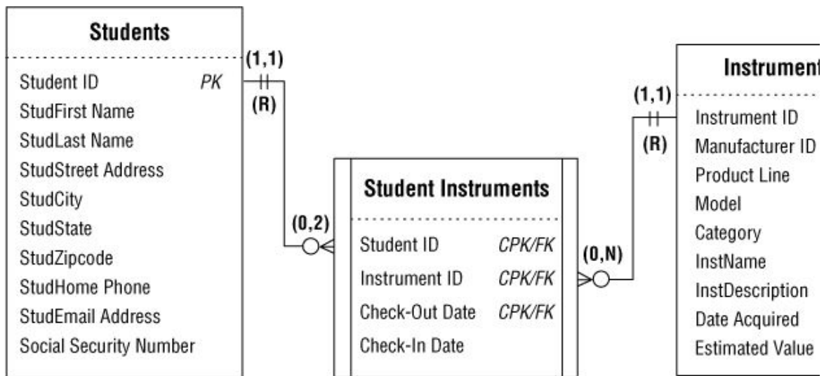
Figure 11.1. Tables from the Bel Air High School and Lake City High School databases
