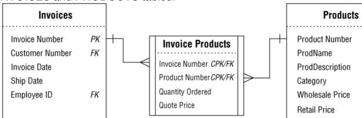
Figure 10.67. Establishing and diagramming the many-to-many relationship between the INVOICES and PRODUCTS tables
