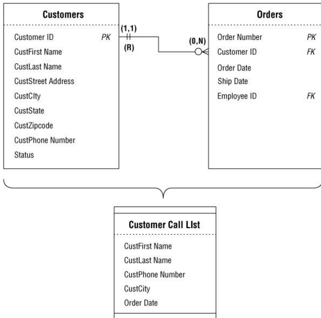
Figure 12.14. View diagram for the CUSTOMER CALL LIST view Using Calculated Fields Where Appropriate
