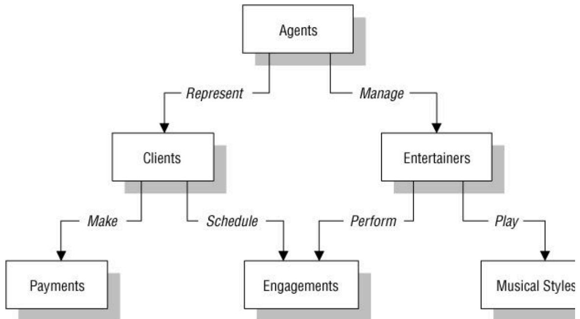
Figure 1.3. Diagram of a typical network database
