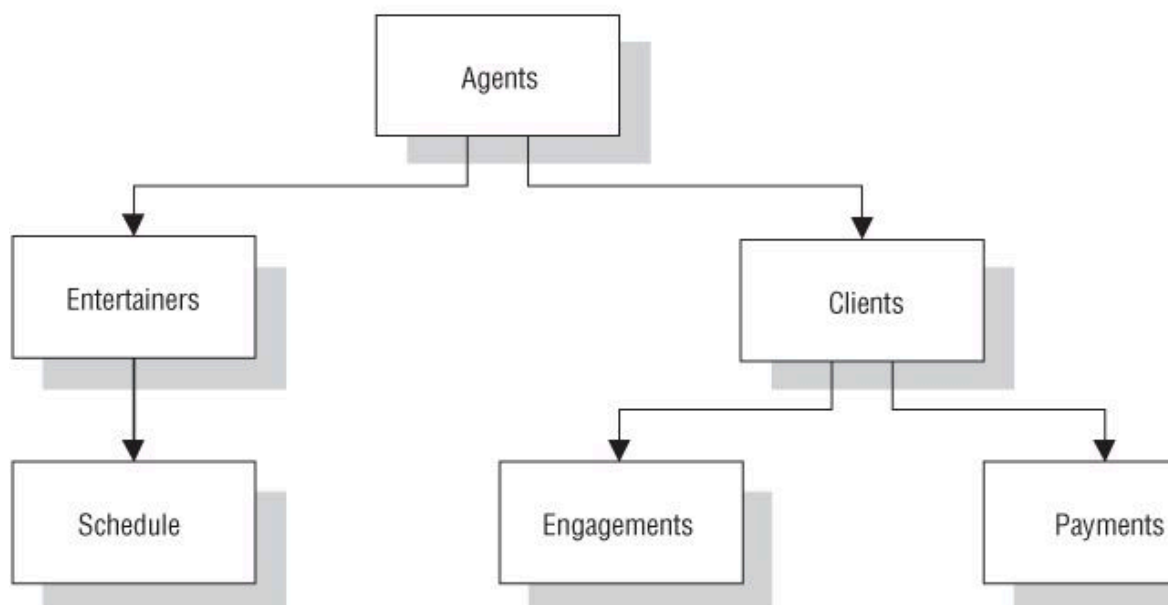
Figure 1.1. Diagram of a typical hierarchical database
