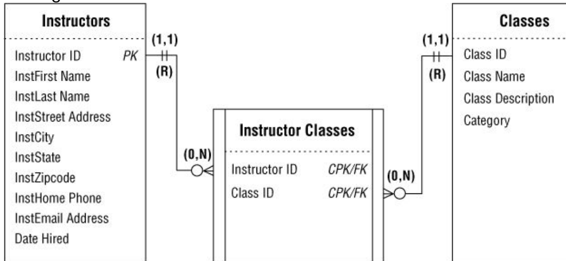
Figure 11.9. A relationship diagram for tables from a dance studio database
