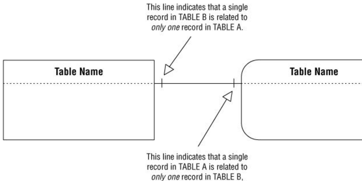
Figure 10.5. Diagramming a one-to-one relationship
