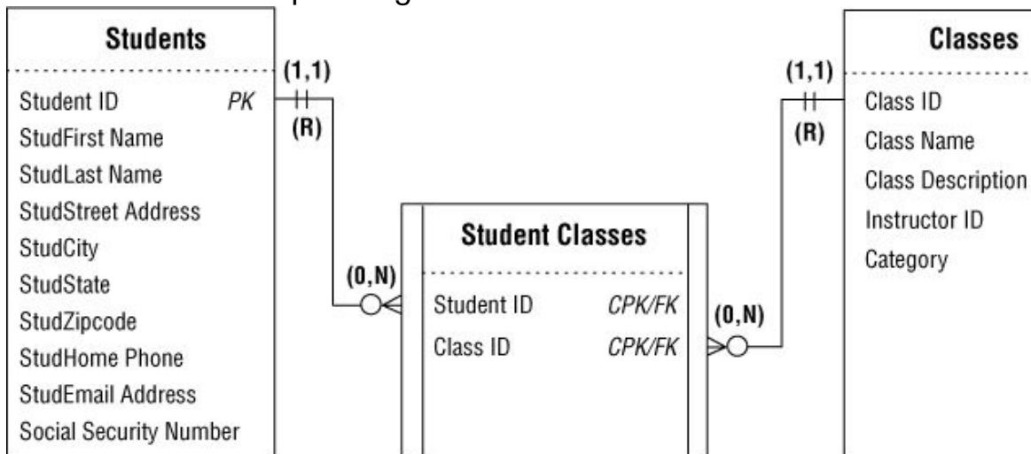
Figure 11.4. Tables and relationships from a school database
