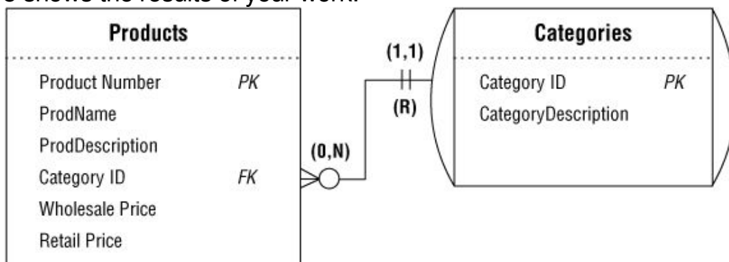
Figure 11.18. The relationship diagram for the PRODUCTS and CATEGORIES tables
