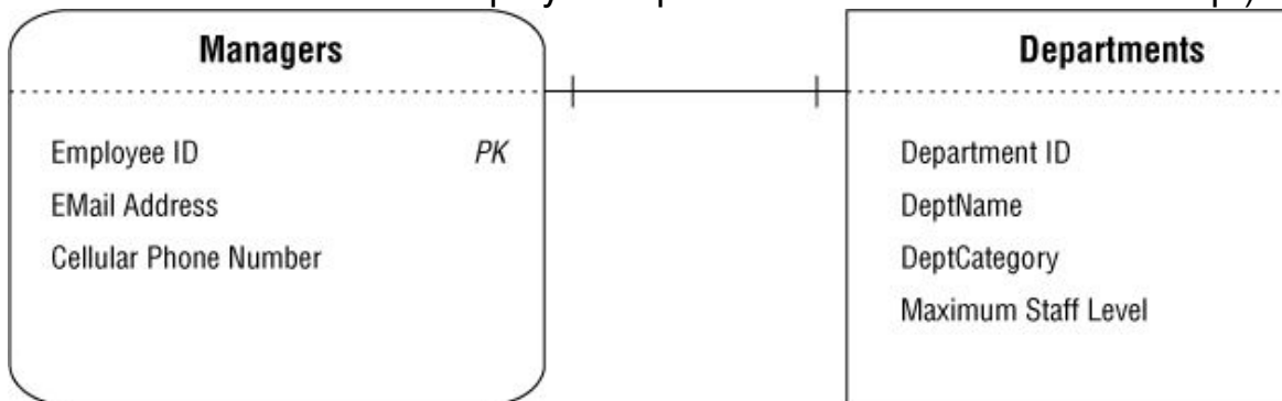
Figure 10.34. A one-to-one relationship with a subset table in the parent role
