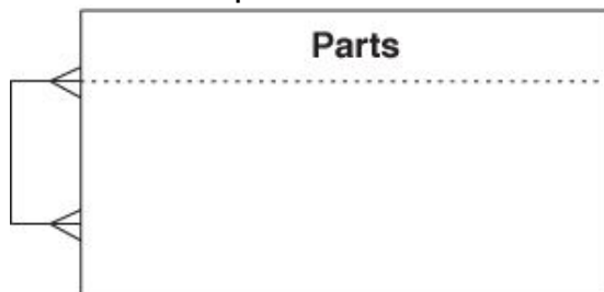
Figure 10.25. Diagramming a self-referencing many-to-many relationship
