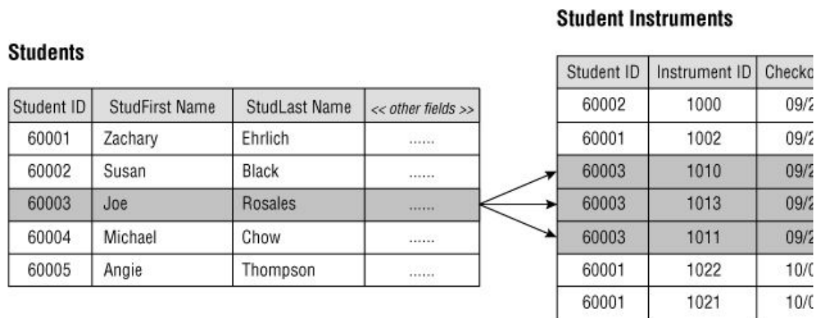
Figure 10.1. A pair of logically related tables
