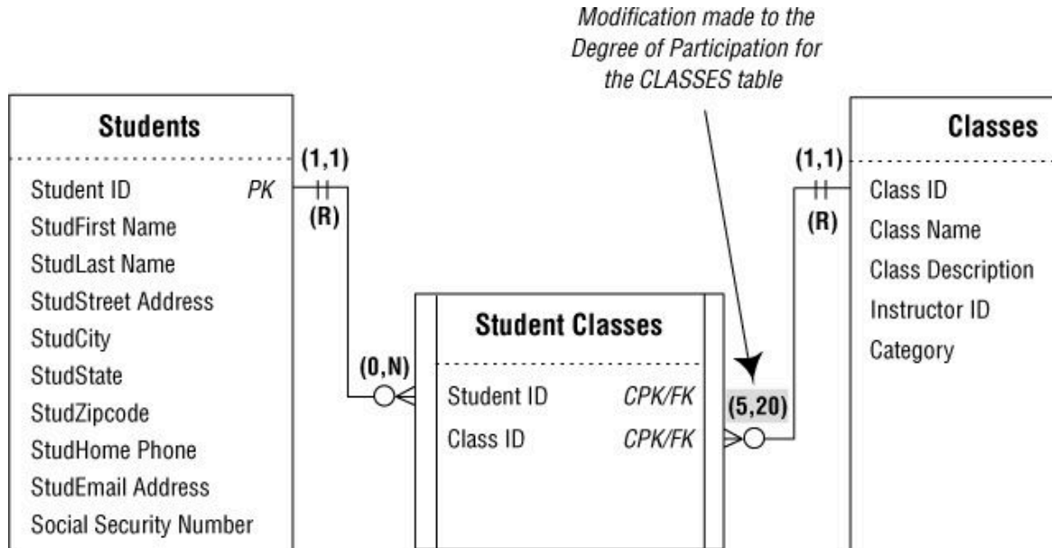
Figure 11.5. Establishing a relationship-specific business rule Defining and Establishing Business Rules
