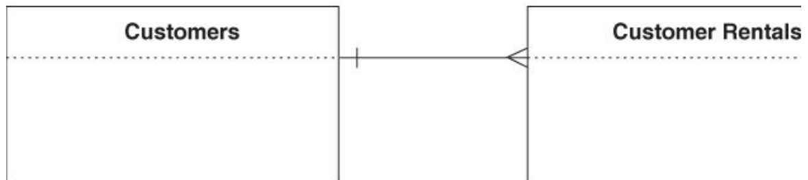
Figure 10.11. The relationship diagram for the CUSTOMERS and CUSTOMER RENTALS tables
