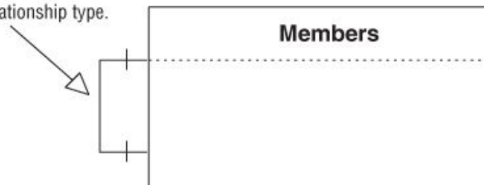
Figure 10.21. Diagramming a self-referencing one-to-one relationship
