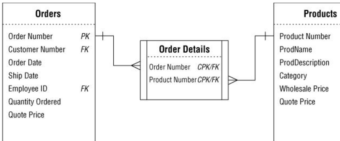
Figure 10.43. Properly establishing the many-to-many relationship between the ORDERS and PRODUCTS tables
