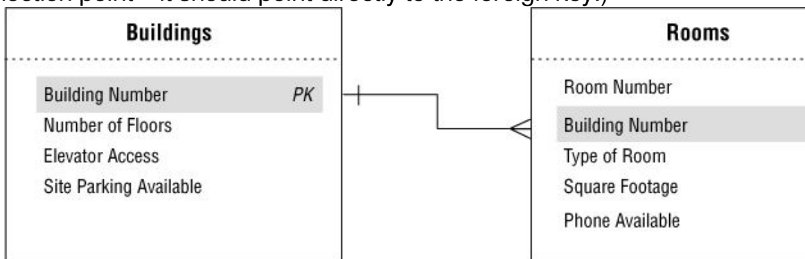
Figure 10.37. Establishing the one-to-many relationship between the BUILDINGS and ROOMS tables
