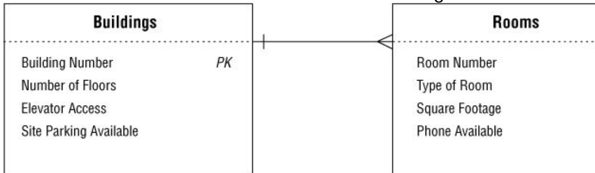
Figure 10.36. The existing one-to-many relationship between the BUILDINGS and ROOMS tables
