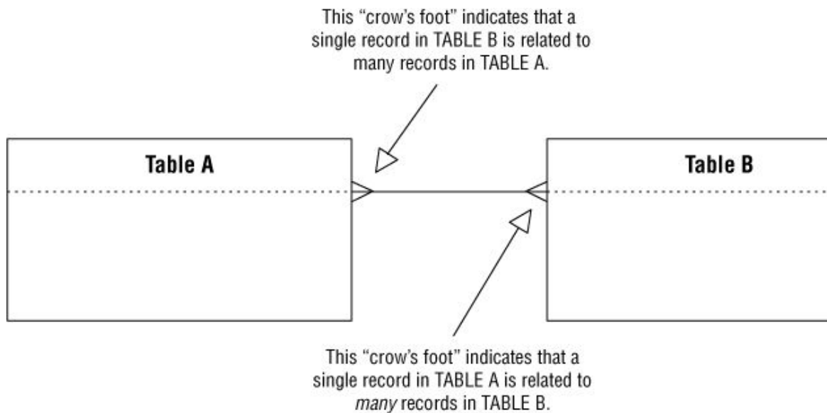
Figure 10.14. Diagramming a many-to-many relationship
