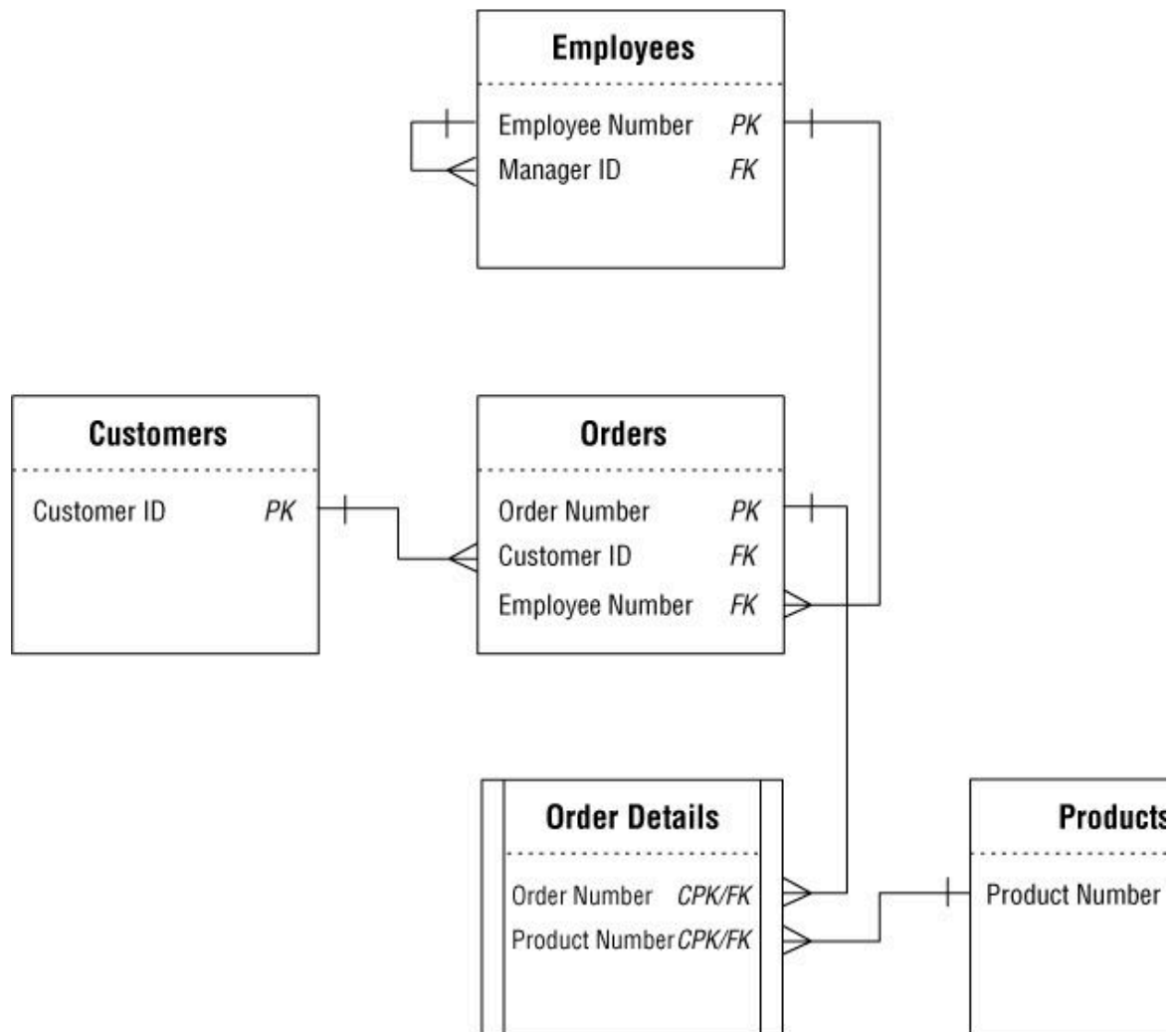
Figure 10.56. What deletion rule is appropriate for a given relationship?
