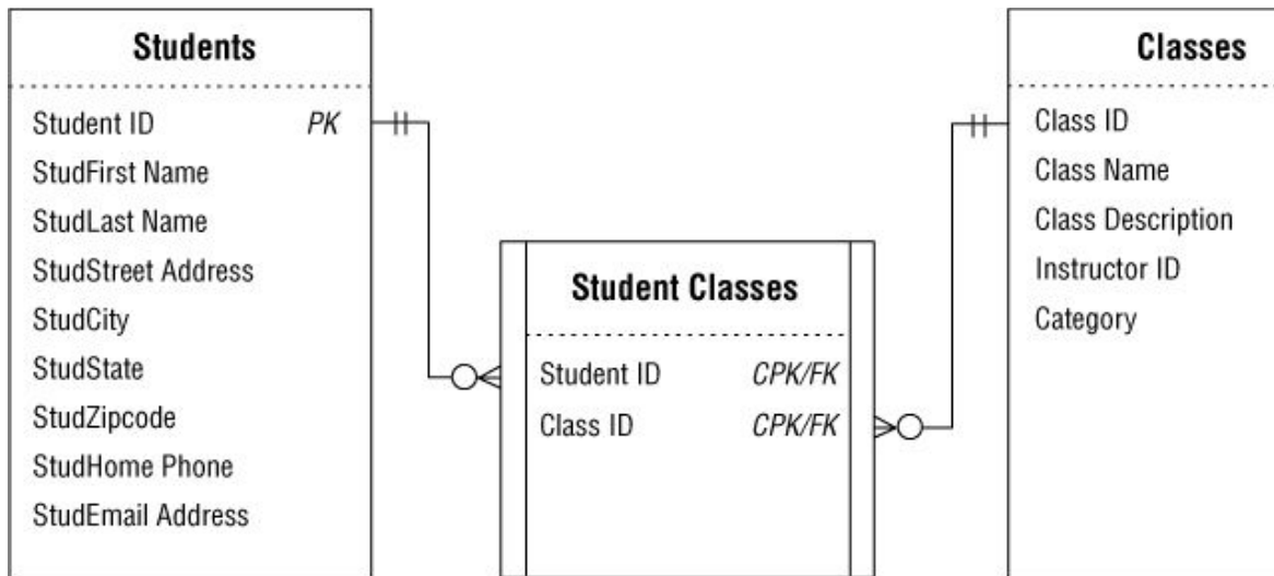
Figure 12.3. Base tables for the CLASS ROSTER view
