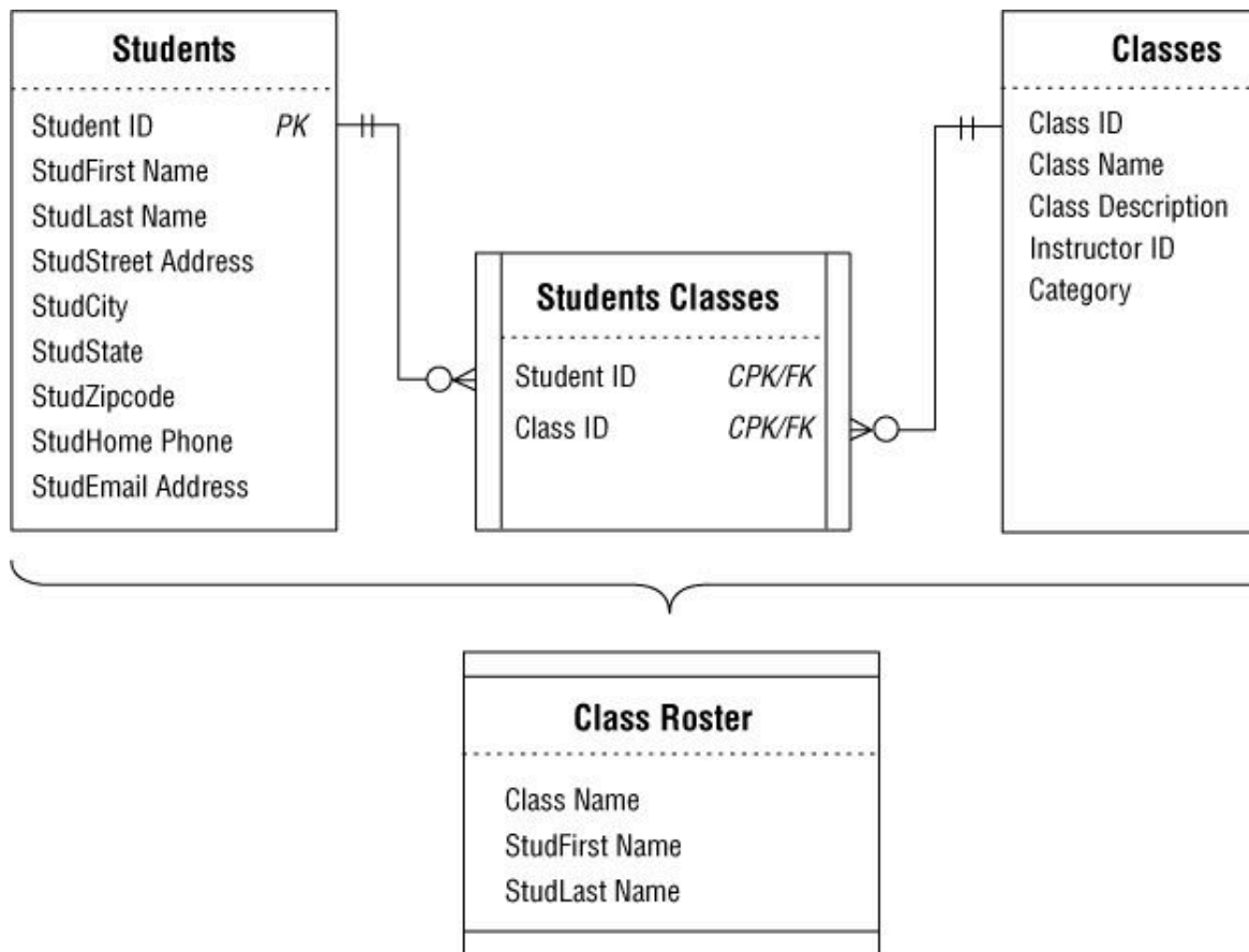
Figure 12.4. The diagram for the CLASS ROSTER view
