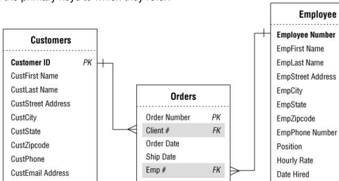
Figure 10.51. Primary keys and foreign keys with mismatched names
