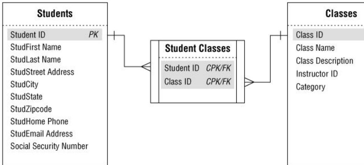
Figure 10.40. Establishing the many-to-many relationship between the STUDENTS and CLASSES tables
