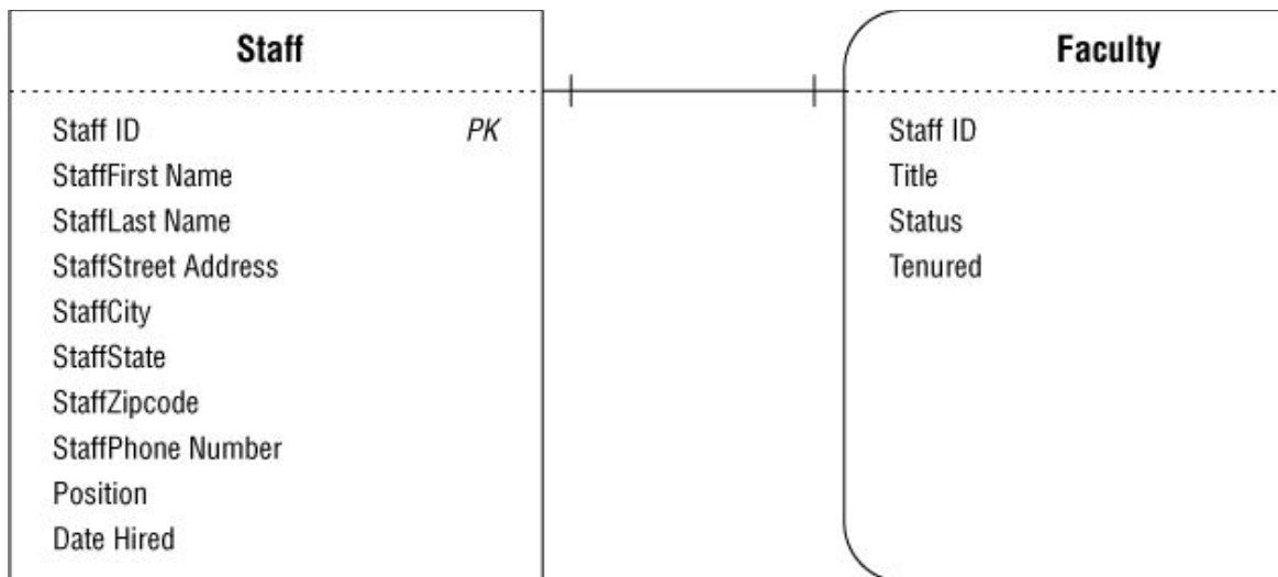
Figure 10.33. Establishing the one-to-one relationship between the STAFF and FACULTY tables
