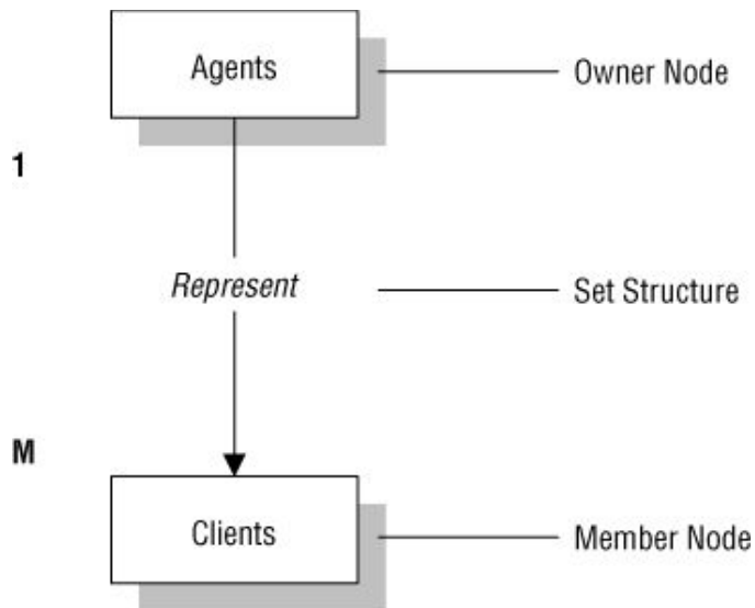
Figure 1.4. A basic set structure
