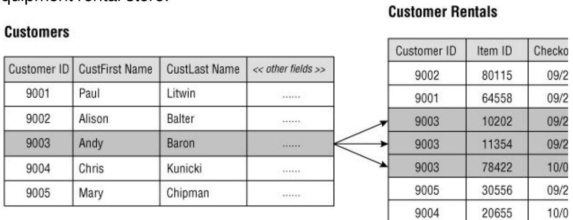
Figure 10.9. A typical example of a one-to-many relationship
