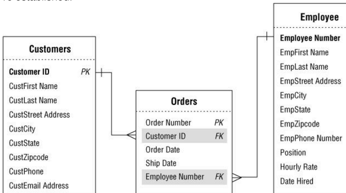
Figure 10.52. Foreign keys that comply with the first element of a foreign key
