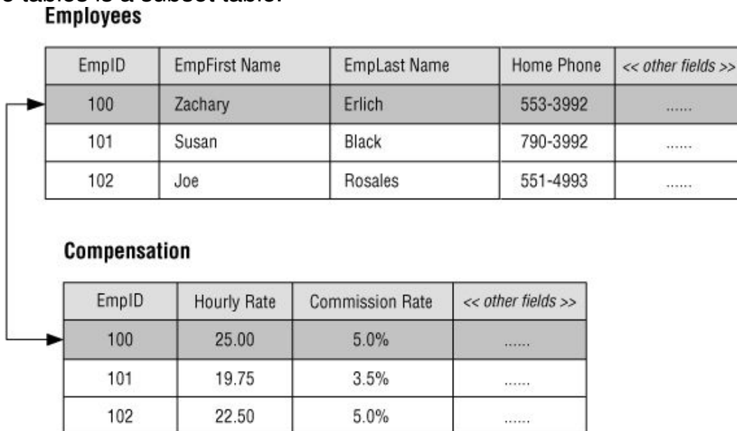
Figure 10.4. A typical example of a one-to-one relationship
