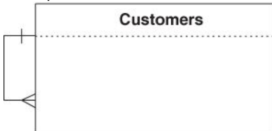
Figure 10.23. Diagramming a self-referencing one-to-many relationship
