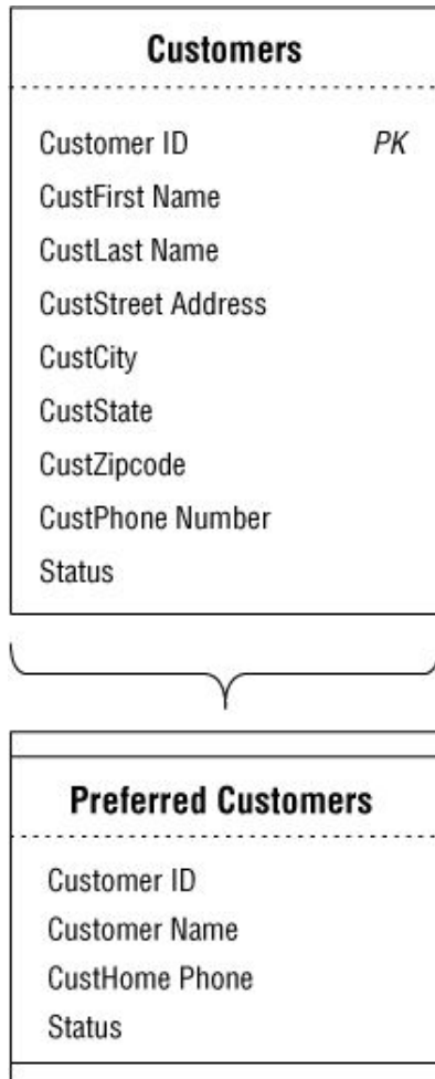
Figure 12.17. View diagram for the PREFERRED CUSTOMERS view
