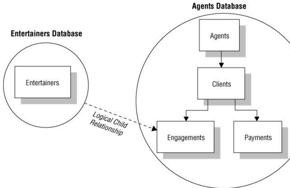
Figure 1.2. Using two hierarchical databases to resolve a many-to-many relationship
