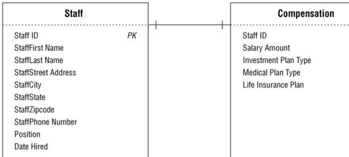
Figure 10.32. Which table would you pick as the parent table?
