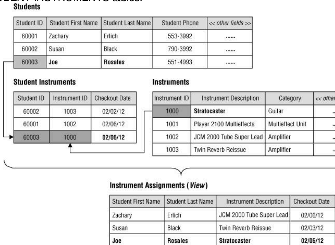
Figure 3.10. An example of a typical view
