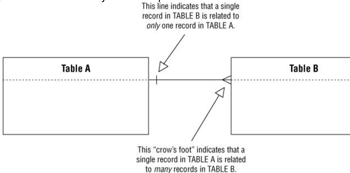
Figure 10.10. Diagramming a one-to-many relationship
