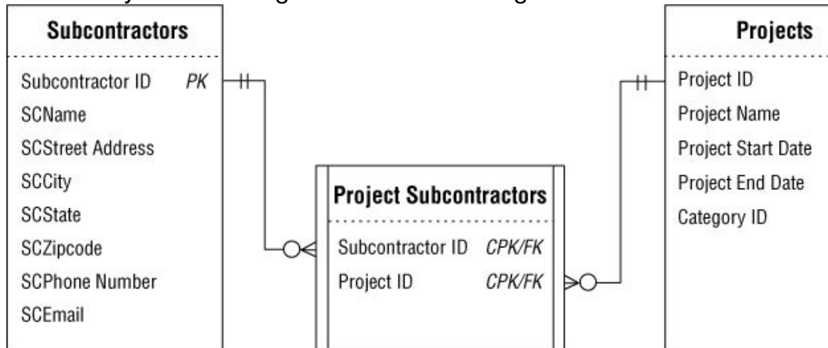
Figure 12.10. Tables from a database for a small contractor
