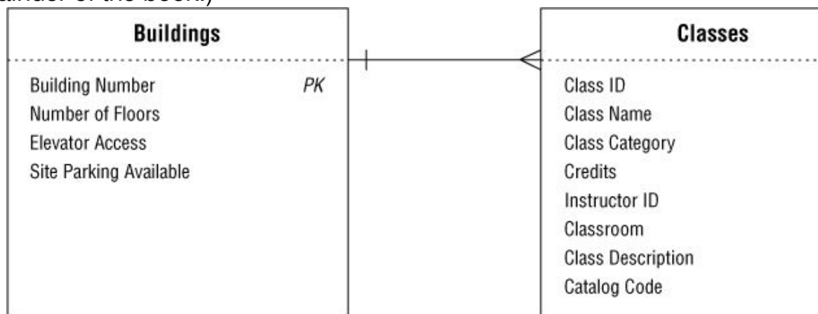
Figure 10.30. Displaying each table’s structure in a relationship diagram
