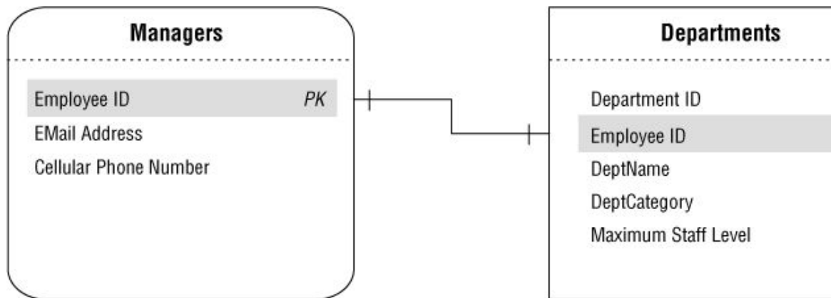
Figure 10.35. Establishing the relationship between the MANAGERS and DEPARTMENTS tables
