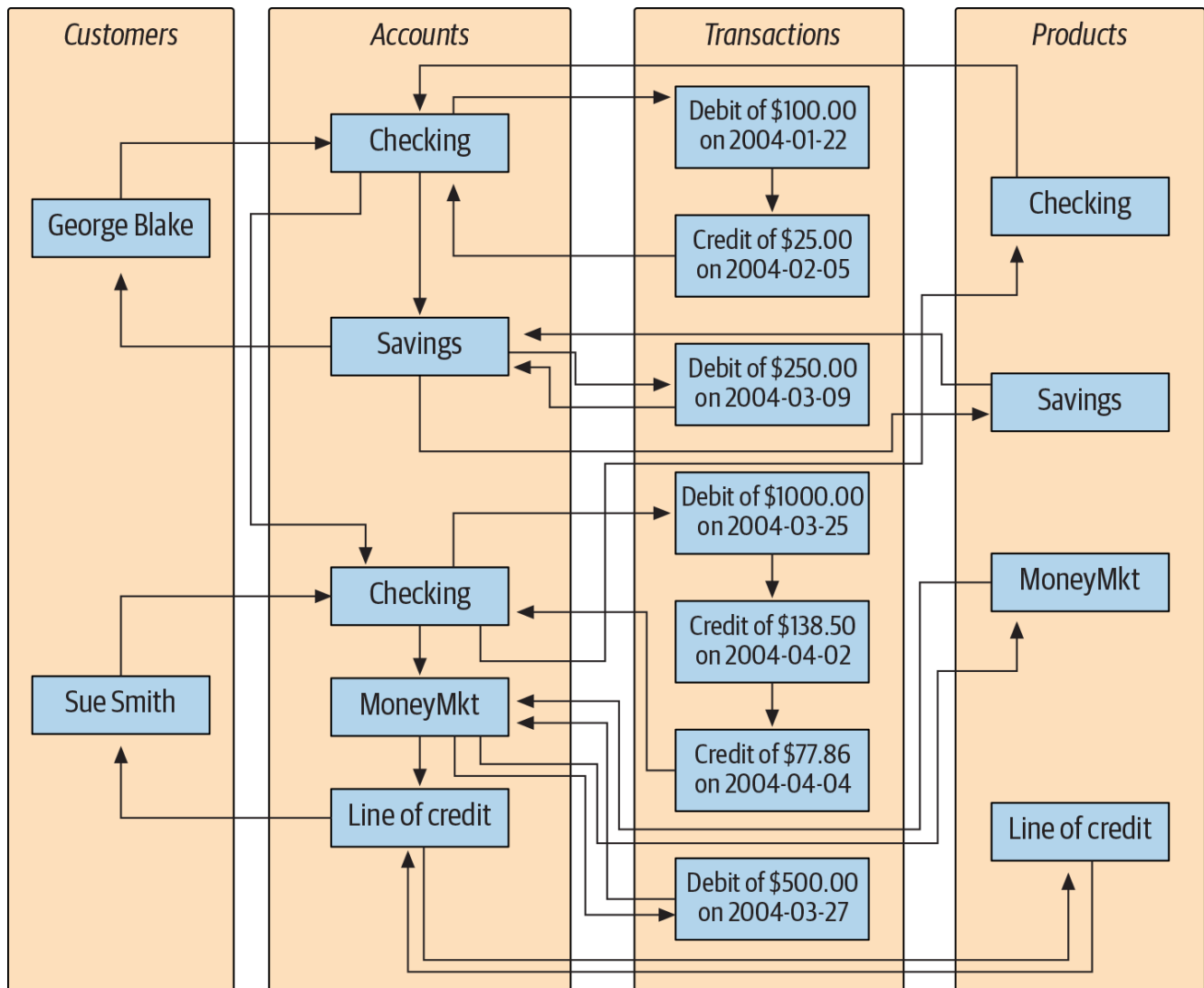
Figure 1-2. Network view of account data
