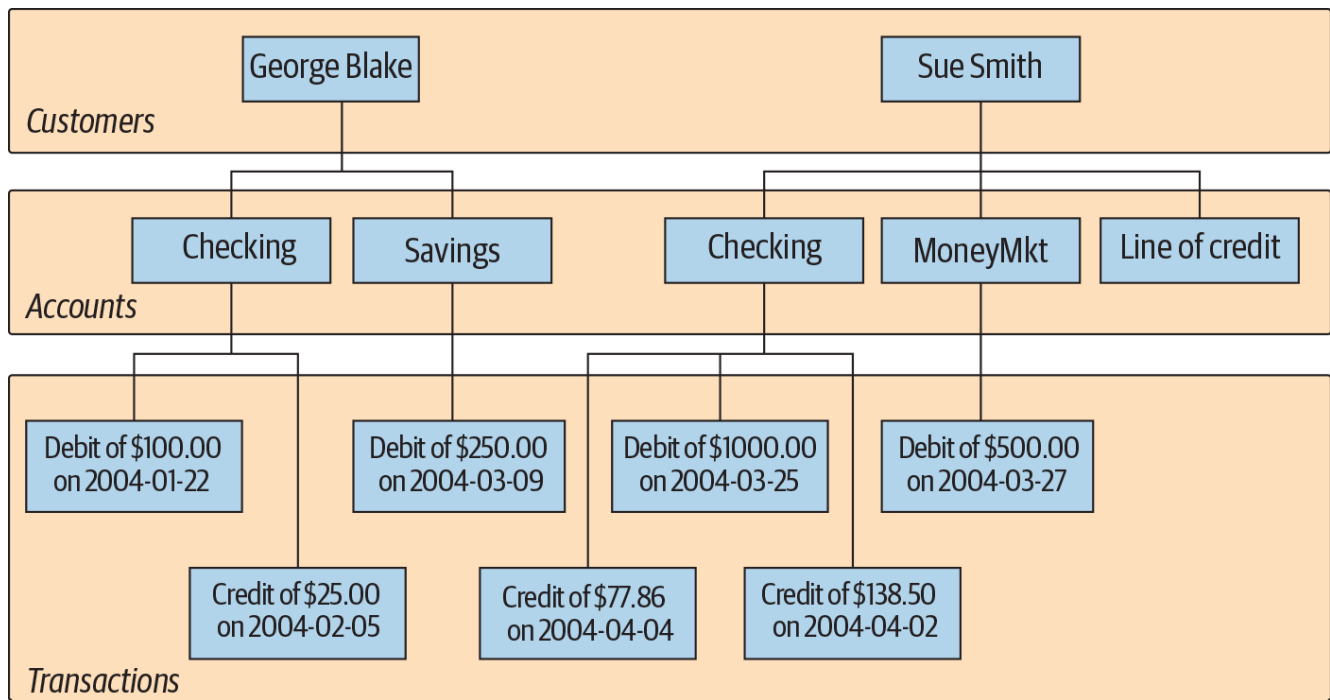
Figure 1-1. Hierarchical view of account data
