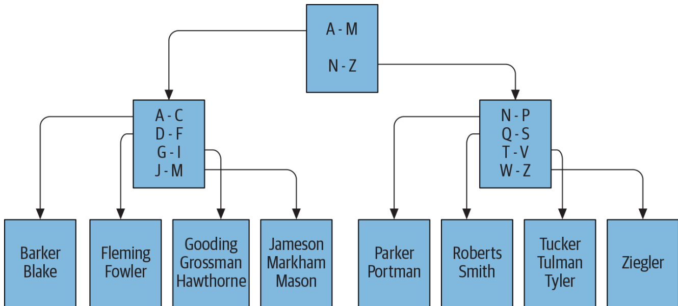
Figure 13-1. B-tree example
