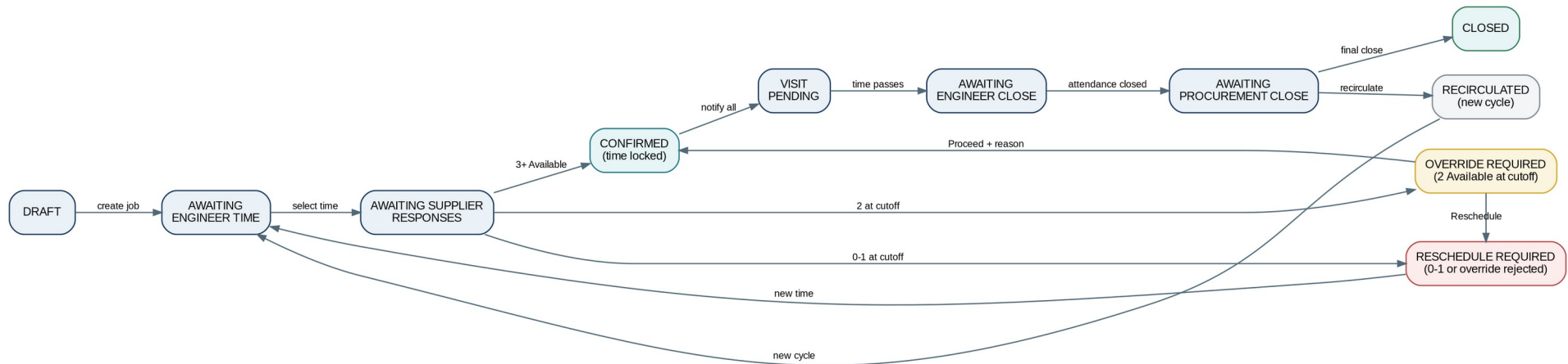
Figure 6: Recommended job-cycle status transitions.
