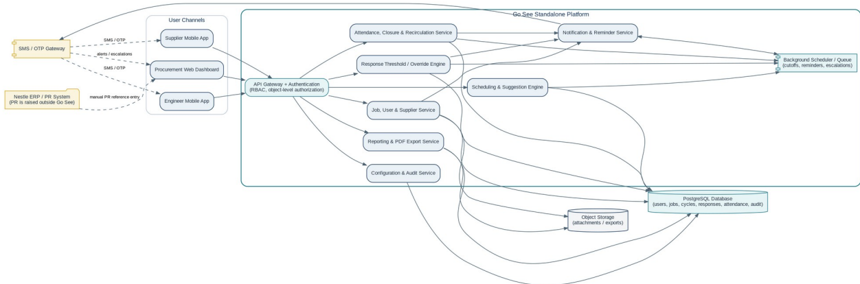
Figure 1: High-level standalone architecture and boundary with the Nestle PR system.
