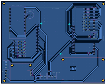
(a) PCB Layout (KiCad PCB Editor)
