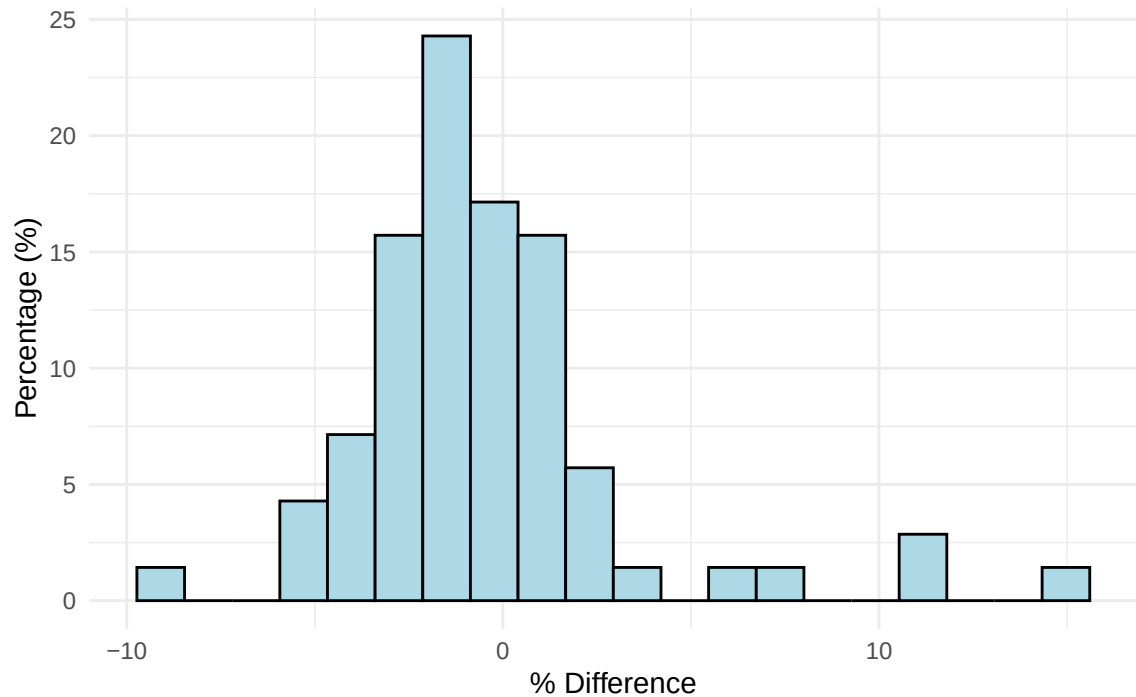
Distribution of % difference for K-138CP-15
