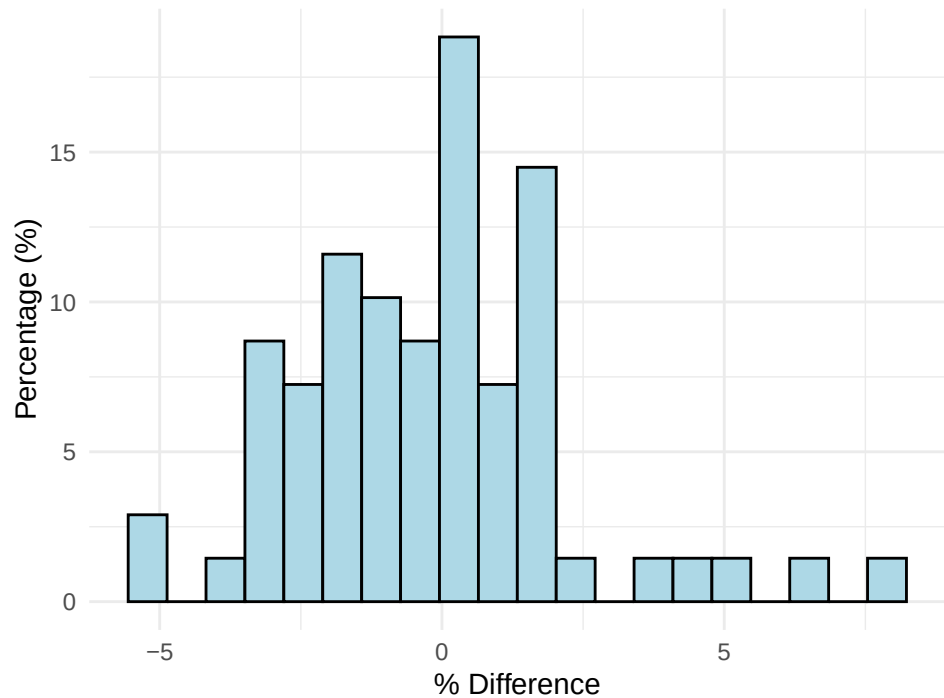
Distribution of % difference for K-148CP-17
