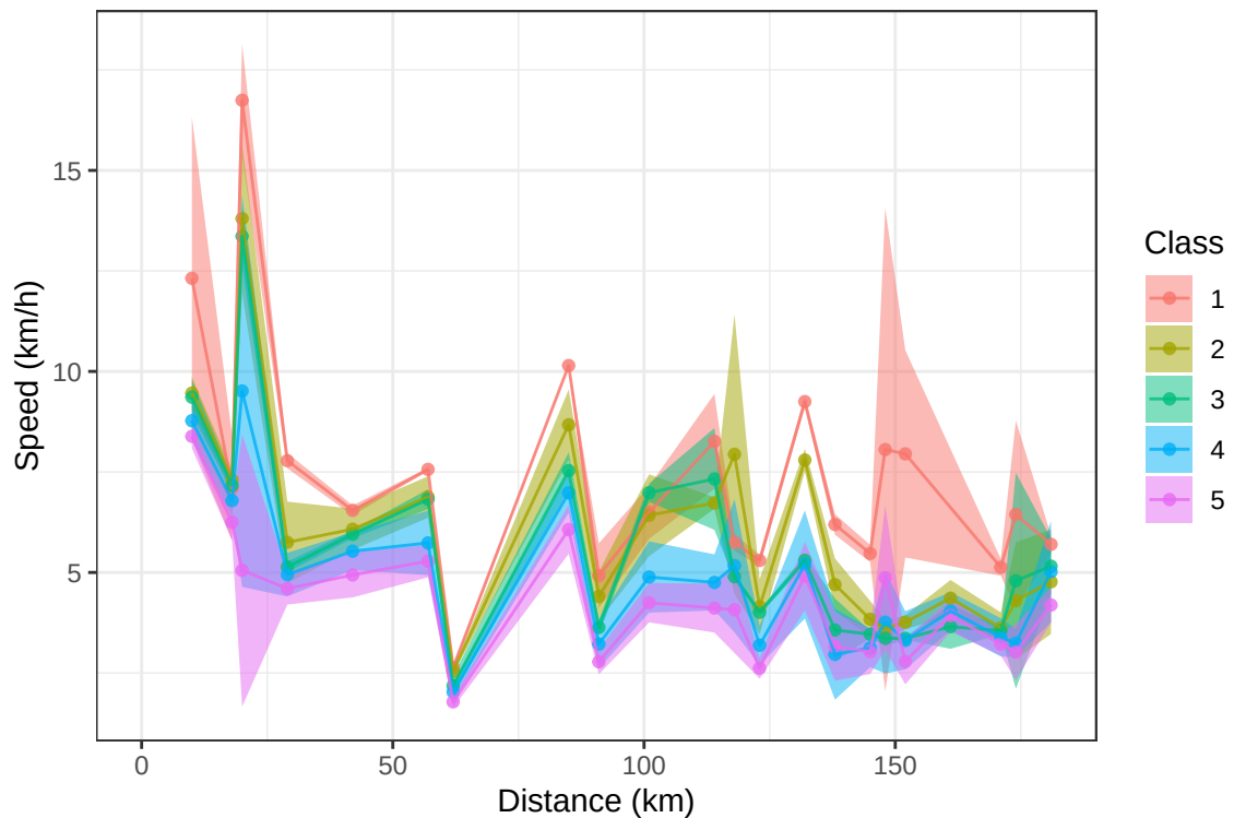
Figure 3: Comparison of the speeds over distance in each split for all models, the ribbon around each line is \pm 1 \sigma .
