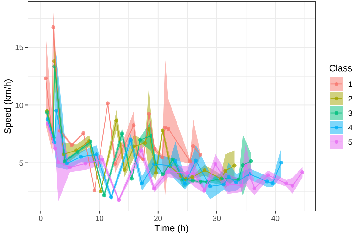
Figure 2: Comparison of the speeds over time, in each split for all models, the ribbon around each line is \pm 1 \sigma .
